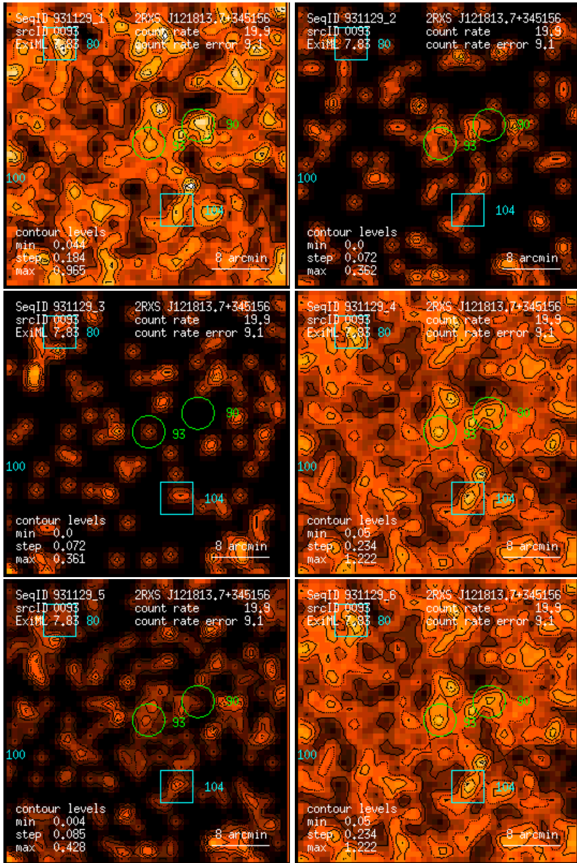
Figure 93: RASS 931129: detection 0093: band rate images, Gaussian filter: (1) PSPC channels 11 – 41, (2) 52 – 90, (3) 91 – 201, (4) 11 – 235, (5) 52 – 201, (6) 11 – 201. Broad band rates in counts/ks. Band rate contour levels in counts/ks/arcmin 2 .
