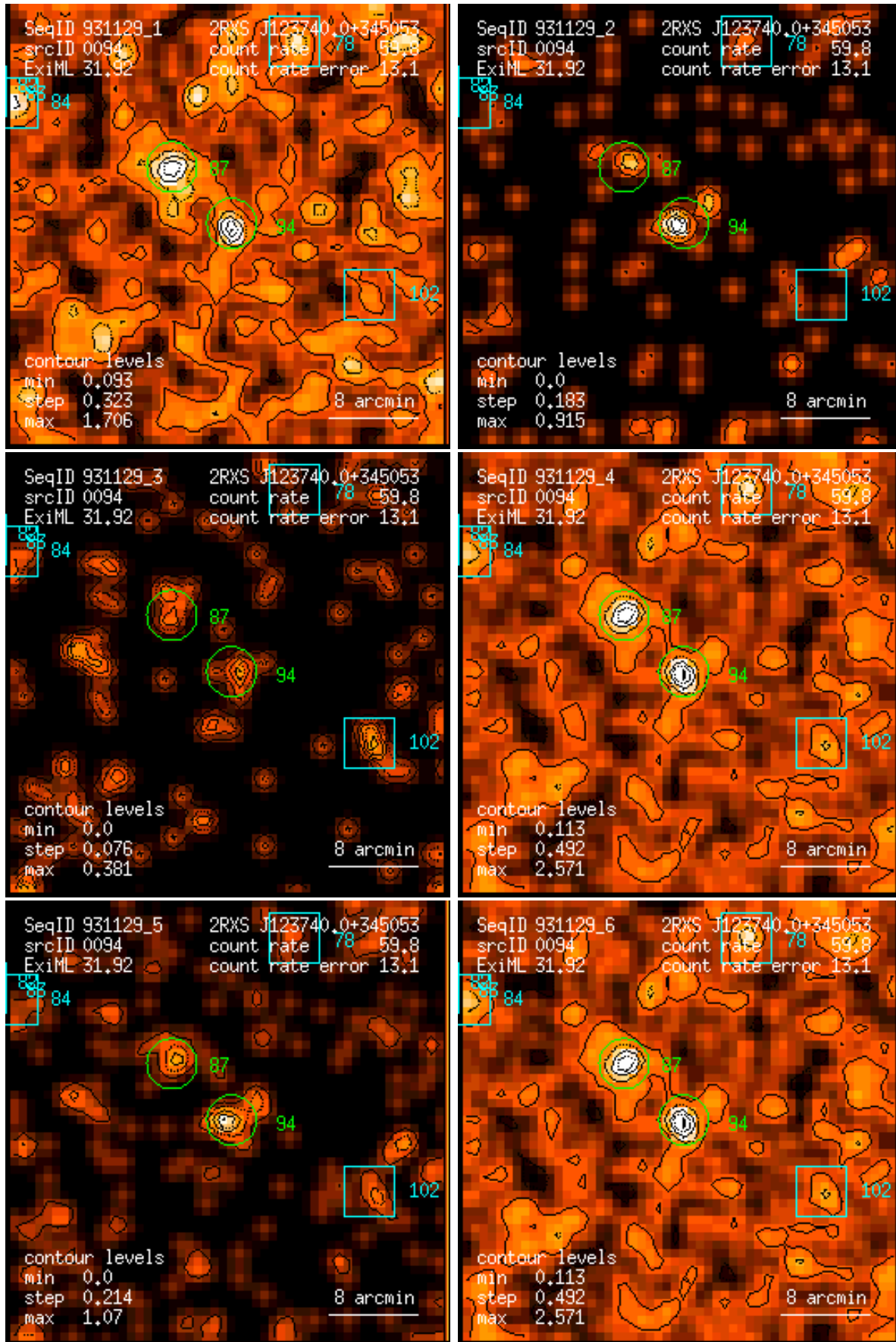
Figure 94: RASS 931129: detection 0094: band rate images, Gaussian filter: (1) PSPC channels 11 – 41, (2) 52 – 90, (3) 91 – 201, (4) 11 – 235, (5) 52 – 201, (6) 11 – 201. Broad band rates in counts/ks. Band rate contour levels in counts/ks/arcmin 2 .
