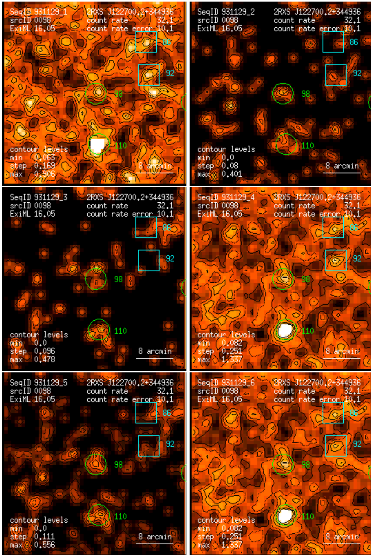
Figure 98: RASS 931129: detection 0098: band rate images, Gaussian filter: (1) PSPC channels 11 – 41, (2) 52 – 90, (3) 91 – 201, (4) 11 – 235, (5) 52 – 201, (6) 11 – 201. Broad band rates in counts/ks. Band rate contour levels in counts/ks/arcmin 2 .
