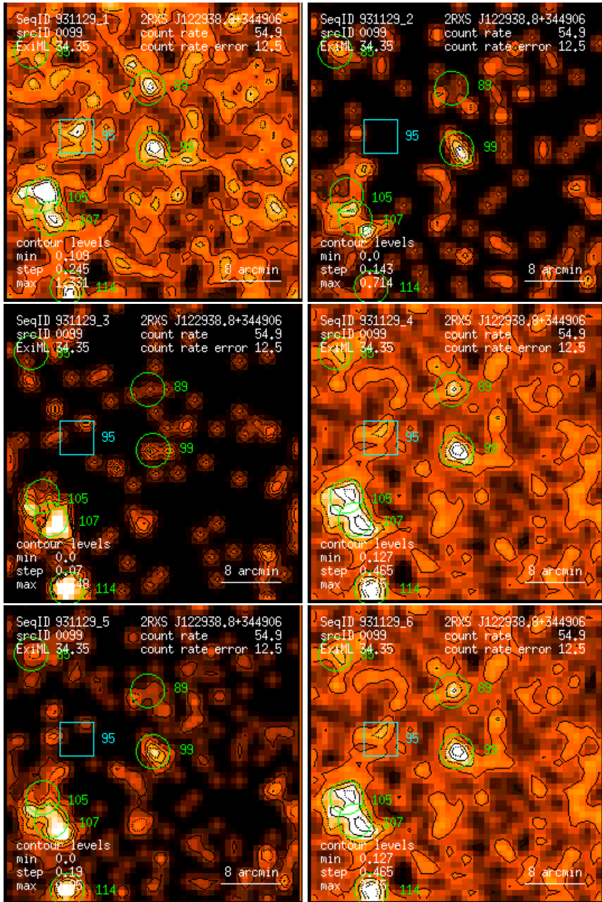
Figure 99: RASS 931129: detection 0099: band rate images, Gaussian filter: (1) PSPC channels 11 – 41, (2) 52 – 90, (3) 91 – 201, (4) 11 – 235, (5) 52 – 201, (6) 11 – 201. Broad band rates in counts/ks. Band rate contour levels in counts/ks/arcmin 2 .
