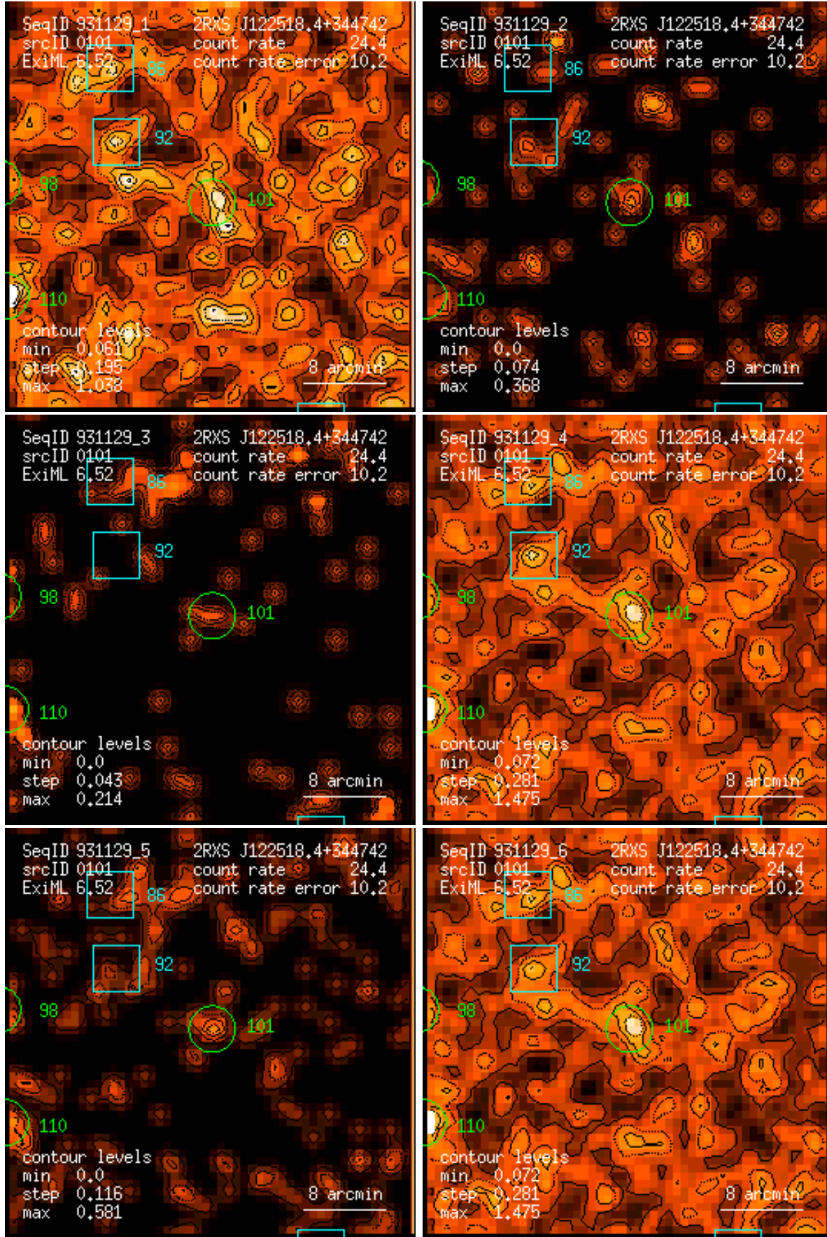
Figure 101: RASS 931129: detection 0101: band rate images, Gaussian filter: (1) PSPC channels 11 – 41, (2) 52 – 90, (3) 91 – 201, (4) 11 – 235, (5) 52 – 201, (6) 11 – 201. Broad band rates in counts/ks. Band rate contour levels in counts/ks/arcmin 2 .
