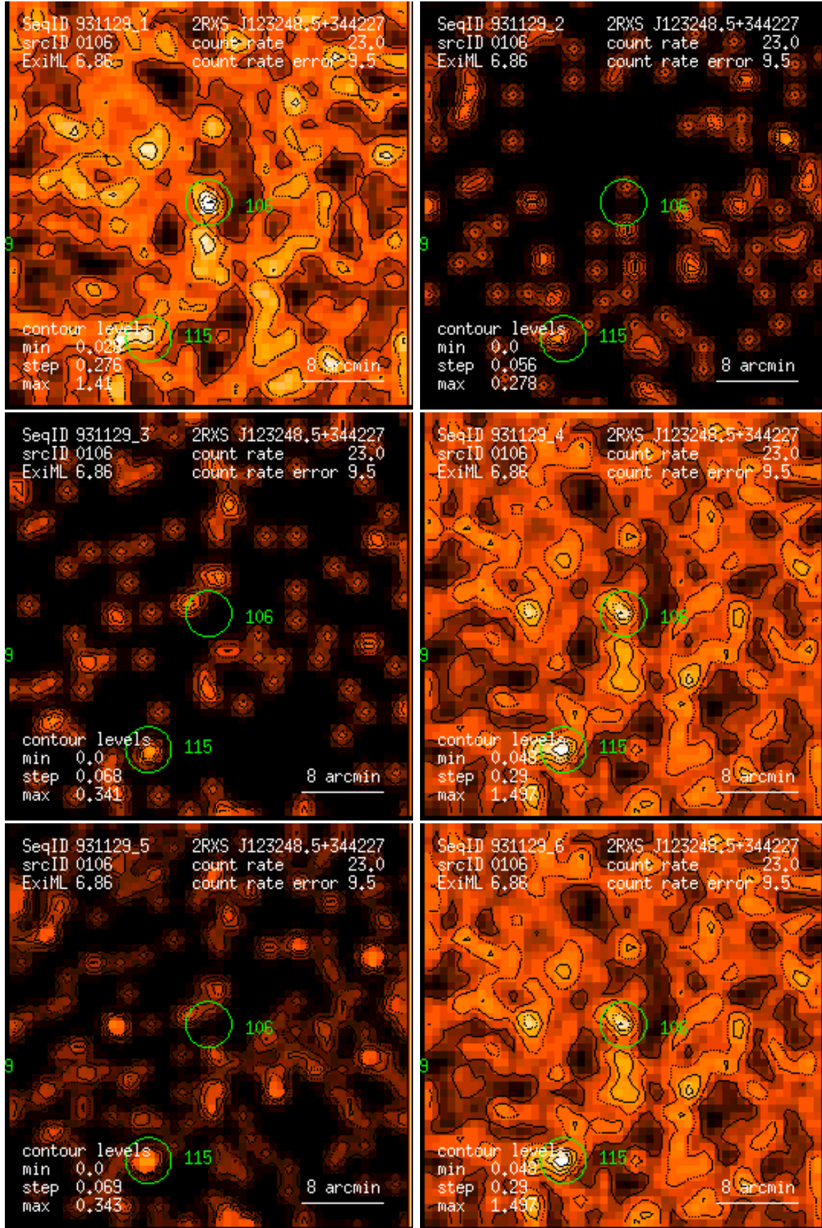
Figure 106: RASS 931129: detection 0106: band rate images, Gaussian filter: (1) PSPC channels 11 – 41, (2) 52 – 90, (3) 91 – 201, (4) 11 – 235, (5) 52 – 201, (6) 11 – 201. Broad band rates in counts/ks. Band rate contour levels in counts/ks/arcmin 2 .
