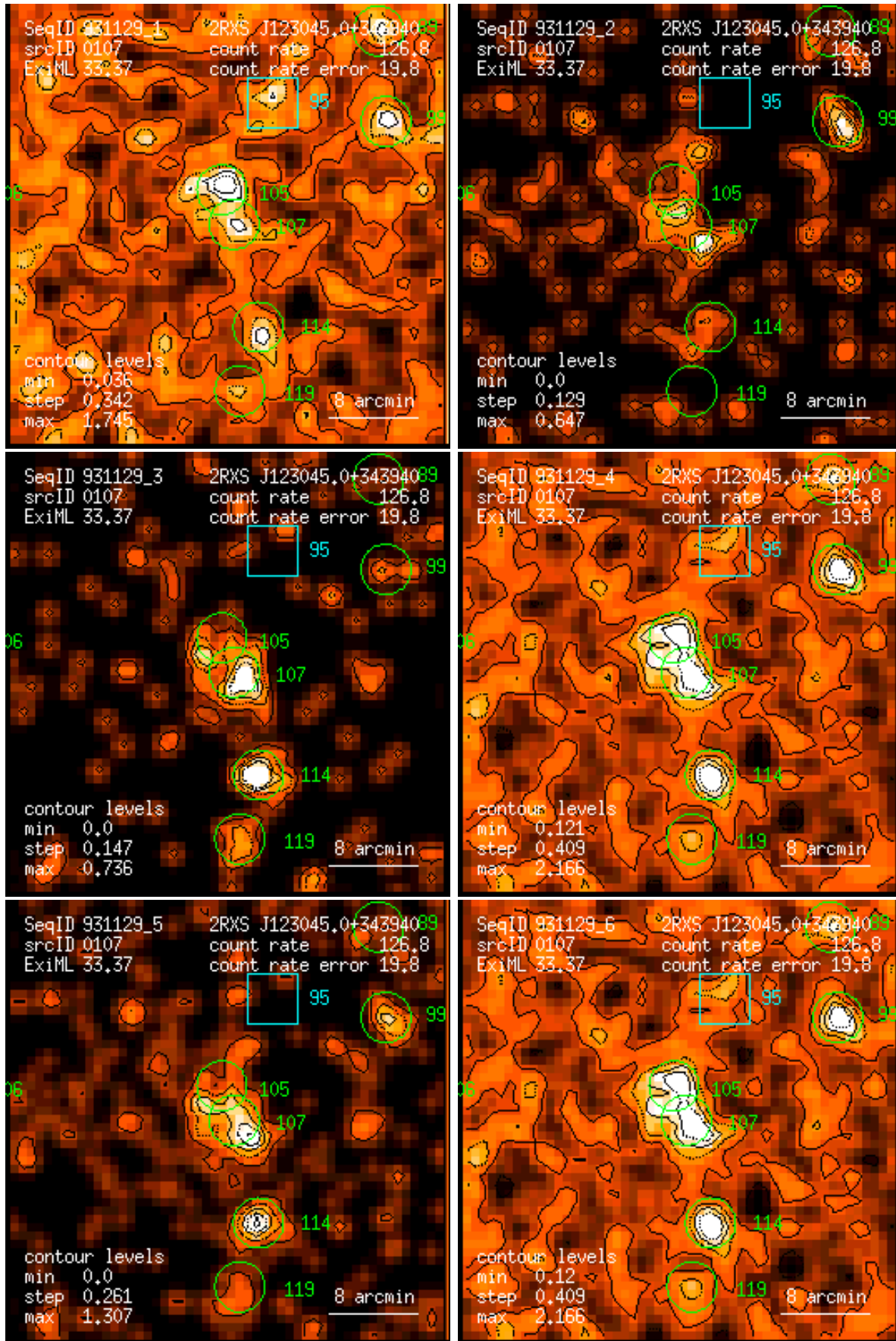
Figure 107: RASS 931129: detection 0107: band rate images, Gaussian filter: (1) PSPC channels 11 – 41, (2) 52 – 90, (3) 91 – 201, (4) 11 – 235, (5) 52 – 201, (6) 11 – 201. Broad band rates in counts/ks. Band rate contour levels in counts/ks/arcmin 2 .
