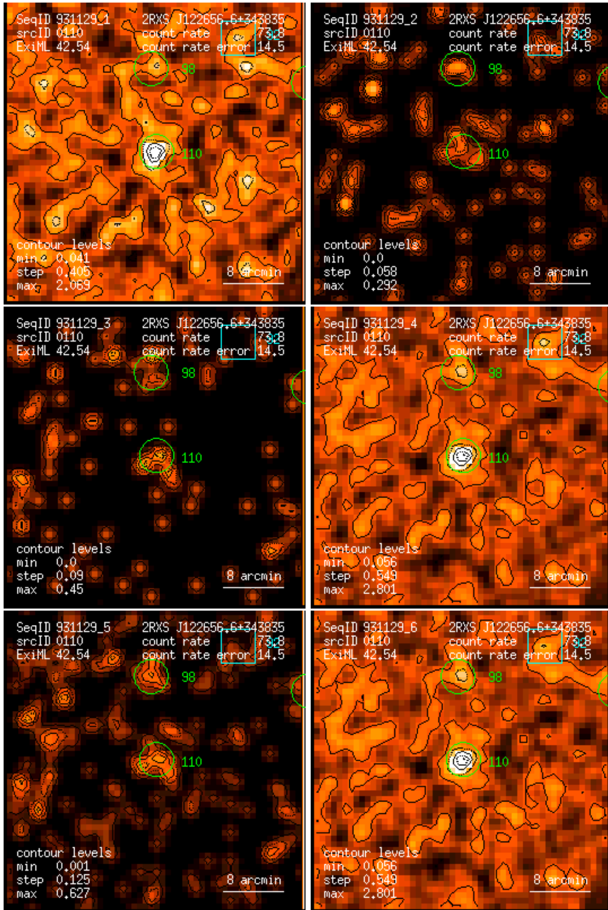
Figure 110: RASS 931129: detection 0110: band rate images, Gaussian filter: (1) PSPC channels 11 – 41, (2) 52 – 90, (3) 91 – 201, (4) 11 – 235, (5) 52 – 201, (6) 11 – 201. Broad band rates in counts/ks. Band rate contour levels in counts/ks/arcmin 2 .
