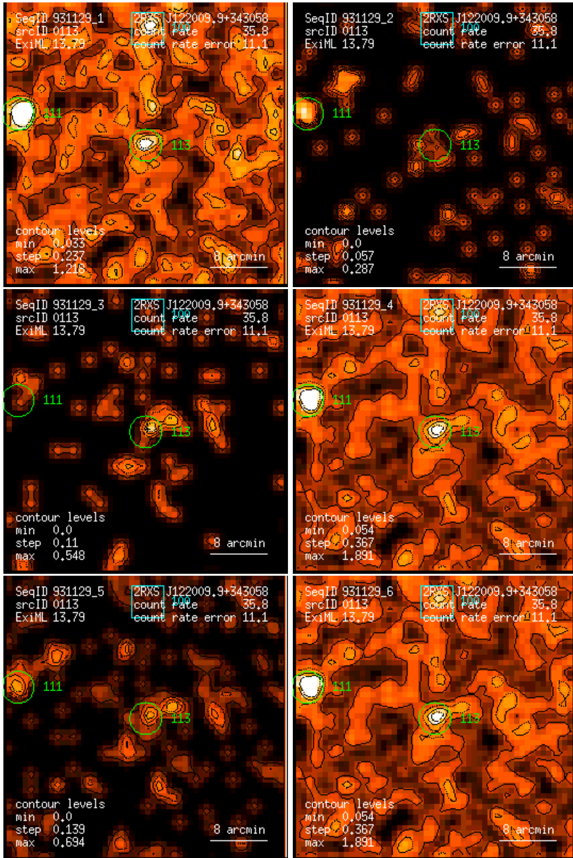
Figure 113: RASS 931129: detection 0113: band rate images, Gaussian filter: (1) PSPC channels 11 – 41, (2) 52 – 90, (3) 91 – 201, (4) 11 – 235, (5) 52 – 201, (6) 11 – 201. Broad band rates in counts/ks. Band rate contour levels in counts/ks/arcmin 2 .
