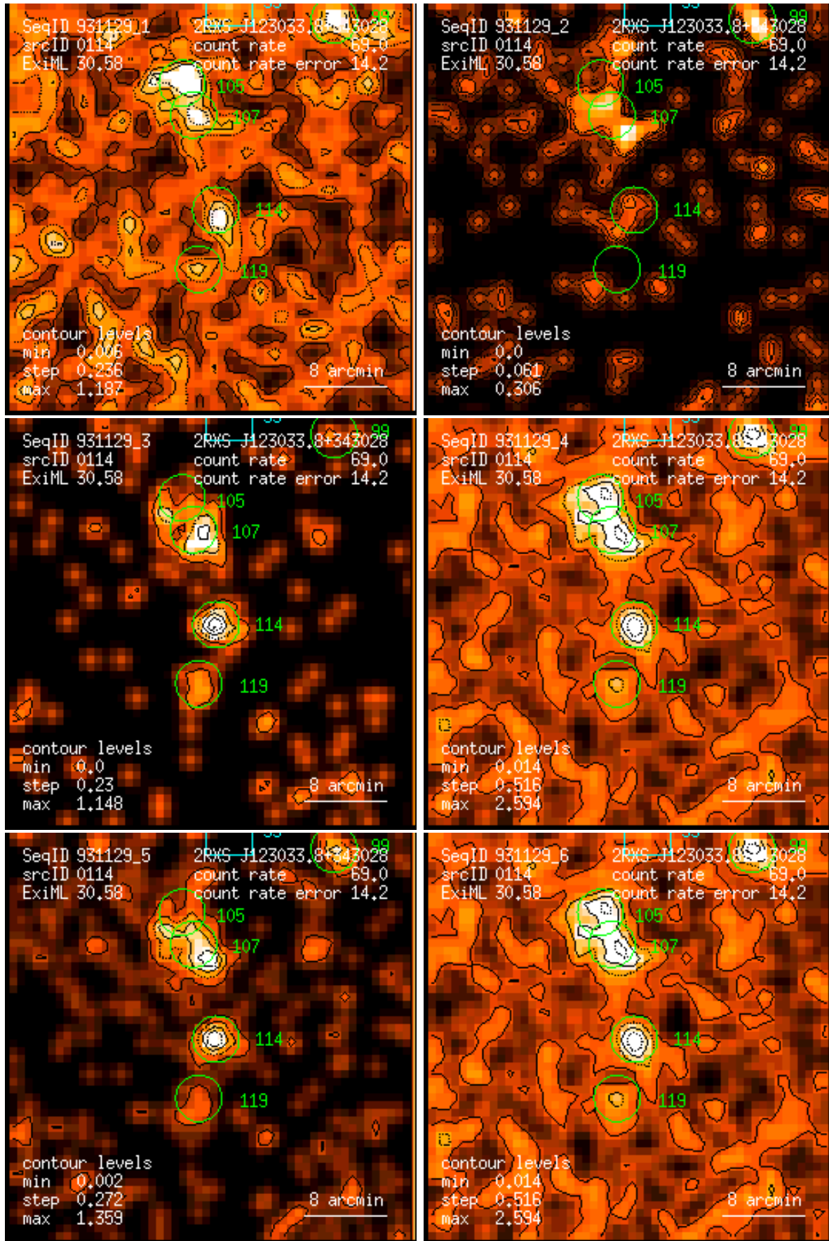
Figure 114: RASS 931129: detection 0114: band rate images, Gaussian filter: (1) PSPC channels 11 – 41, (2) 52 – 90, (3) 91 – 201, (4) 11 – 235, (5) 52 – 201, (6) 11 – 201. Broad band rates in counts/ks. Band rate contour levels in counts/ks/arcmin 2 .
