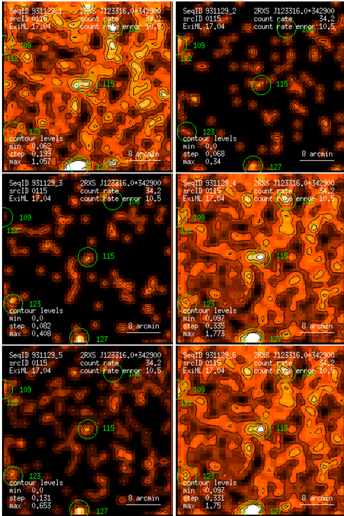
Figure 115: RASS 931129: detection 0115: band rate images, Gaussian filter: (1) PSPC channels 11 – 41, (2) 52 – 90, (3) 91 – 201, (4) 11 – 235, (5) 52 – 201, (6) 11 – 201. Broad band rates in counts/ks. Band rate contour levels in counts/ks/arcmin 2 .
