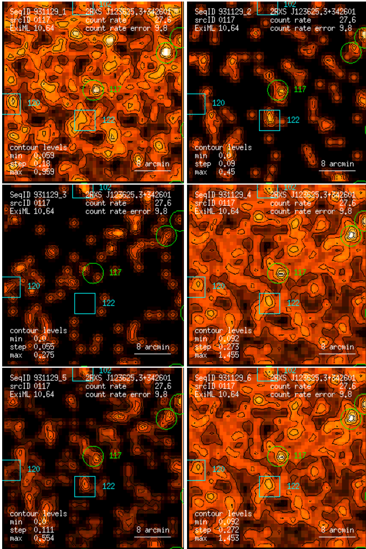
Figure 117: RASS 931129: detection 0117: band rate images, Gaussian filter: (1) PSPC channels 11 – 41, (2) 52 – 90, (3) 91 – 201, (4) 11 – 235, (5) 52 – 201, (6) 11 – 201. Broad band rates in counts/ks. Band rate contour levels in counts/ks/arcmin 2 .
