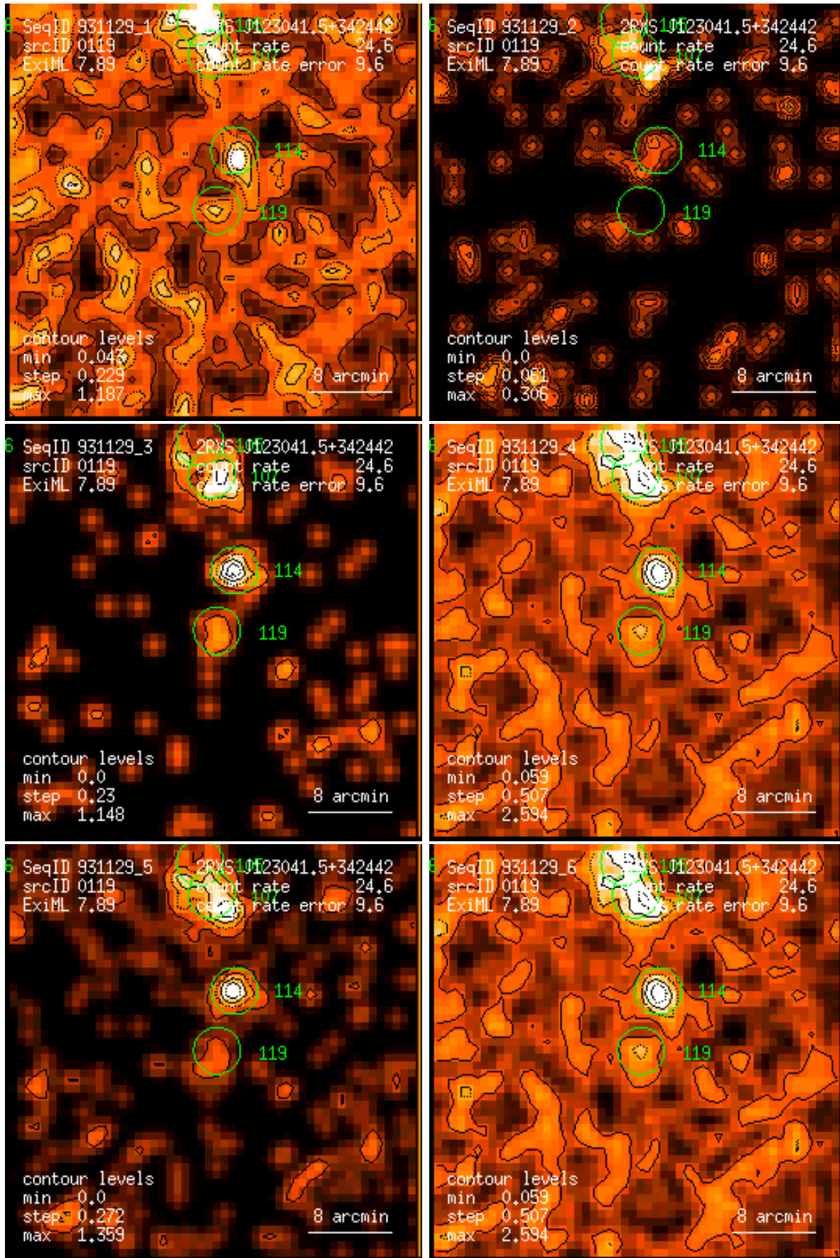
Figure 119: RASS 931129: detection 0119: band rate images, Gaussian filter: (1) PSPC channels 11 – 41, (2) 52 – 90, (3) 91 – 201, (4) 11 – 235, (5) 52 – 201, (6) 11 – 201. Broad band rates in counts/ks. Band rate contour levels in counts/ks/arcmin 2 .
