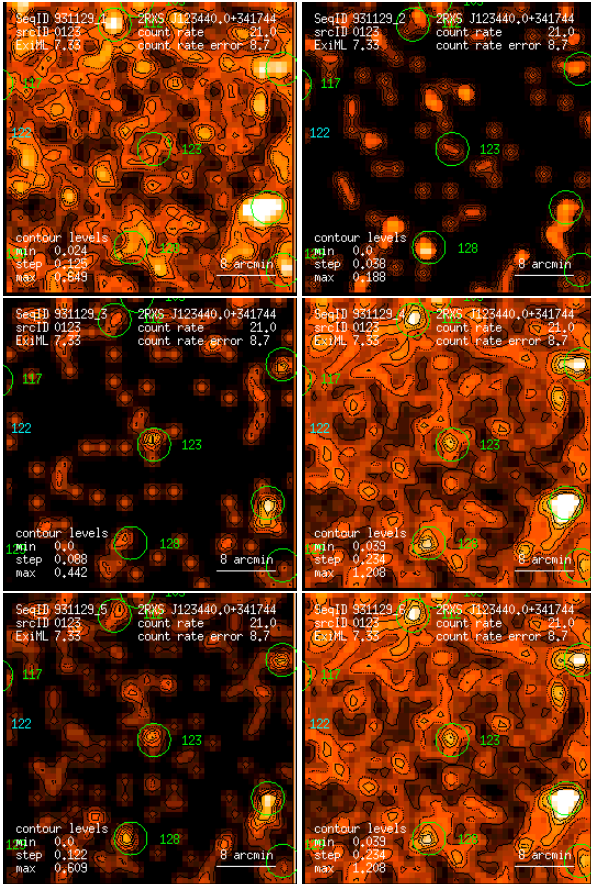
Figure 123: RASS 931129: detection 0123: band rate images, Gaussian filter: (1) PSPC channels 11 – 41, (2) 52 – 90, (3) 91 – 201, (4) 11 – 235, (5) 52 – 201, (6) 11 – 201. Broad band rates in counts/ks. Band rate contour levels in counts/ks/arcmin 2 .
