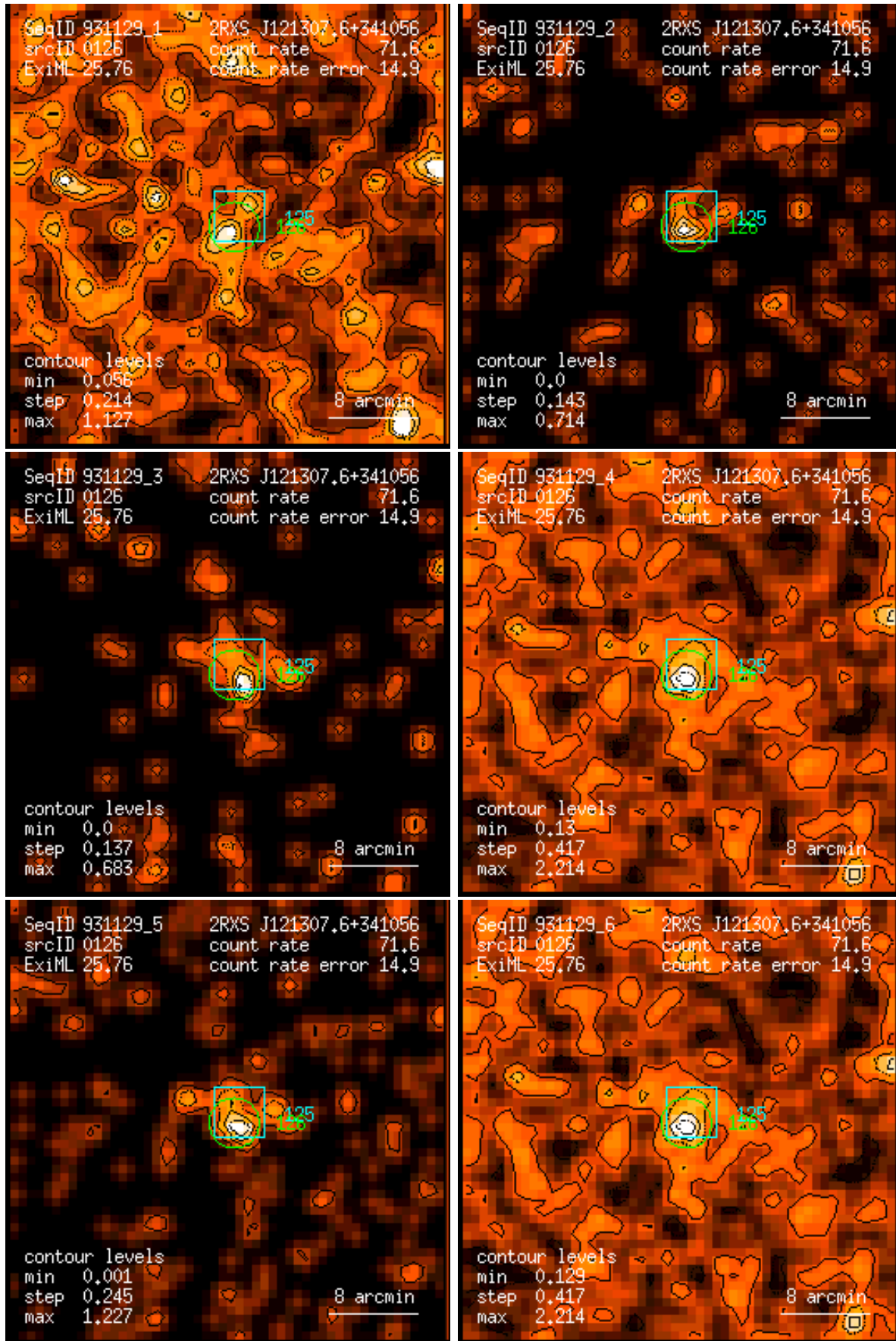
Figure 126: RASS 931129: detection 0126: band rate images, Gaussian filter: (1) PSPC channels 11 – 41, (2) 52 – 90, (3) 91 – 201, (4) 11 – 235, (5) 52 – 201, (6) 11 – 201. Broad band rates in counts/ks. Band rate contour levels in counts/ks/arcmin 2 .
