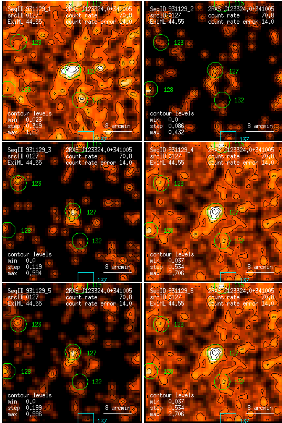
Figure 127: RASS 931129: detection 0127: band rate images, Gaussian filter: (1) PSPC channels 11 – 41, (2) 52 – 90, (3) 91 – 201, (4) 11 – 235, (5) 52 – 201, (6) 11 – 201. Broad band rates in counts/ks. Band rate contour levels in counts/ks/arcmin 2 .
