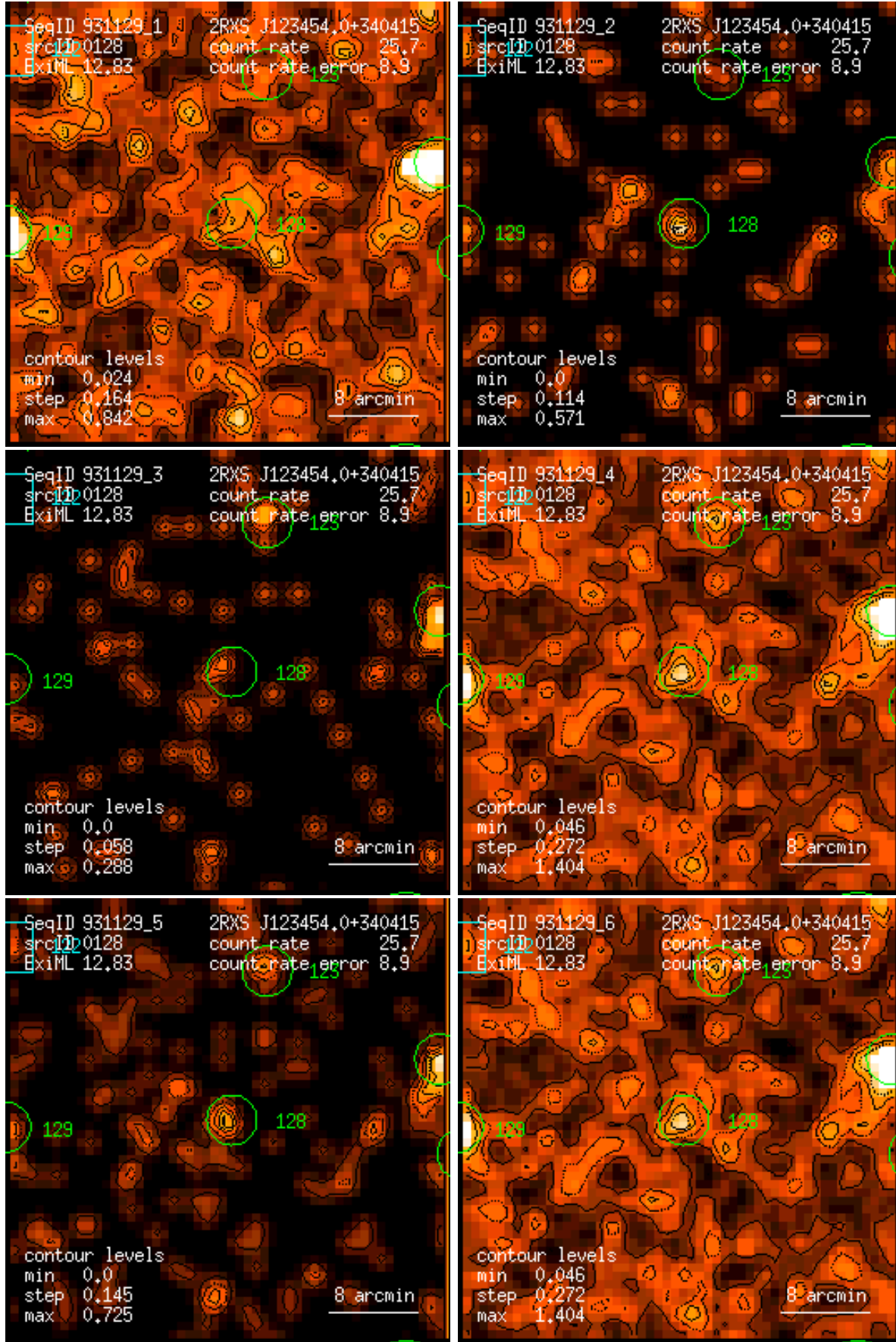
Figure 128: RASS 931129: detection 0128: band rate images, Gaussian filter: (1) PSPC channels 11 – 41, (2) 52 – 90, (3) 91 – 201, (4) 11 – 235, (5) 52 – 201, (6) 11 – 201. Broad band rates in counts/ks. Band rate contour levels in counts/ks/arcmin 2 .
