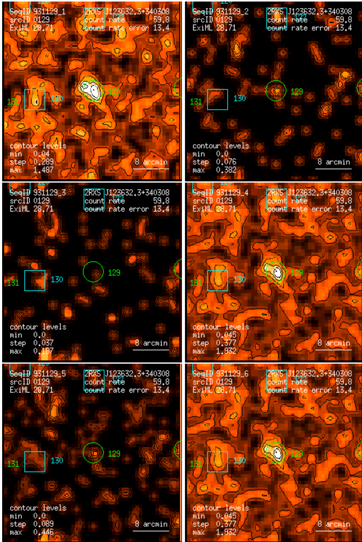
Figure 129: RASS 931129: detection 0129: band rate images, Gaussian filter: (1) PSPC channels 11 – 41, (2) 52 – 90, (3) 91 – 201, (4) 11 – 235, (5) 52 – 201, (6) 11 – 201. Broad band rates in counts/ks. Band rate contour levels in counts/ks/arcmin 2 .
