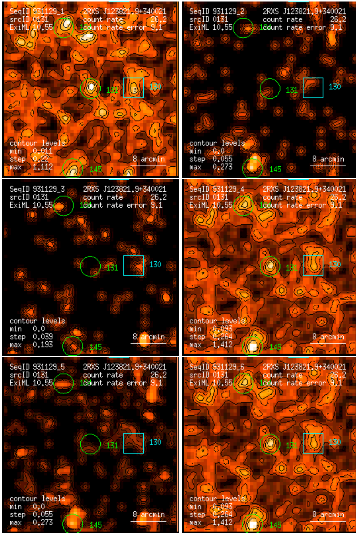
Figure 131: RASS 931129: detection 0131: band rate images, Gaussian filter: (1) PSPC channels 11 – 41, (2) 52 – 90, (3) 91 – 201, (4) 11 – 235, (5) 52 – 201, (6) 11 – 201. Broad band rates in counts/ks. Band rate contour levels in counts/ks/arcmin 2 .
