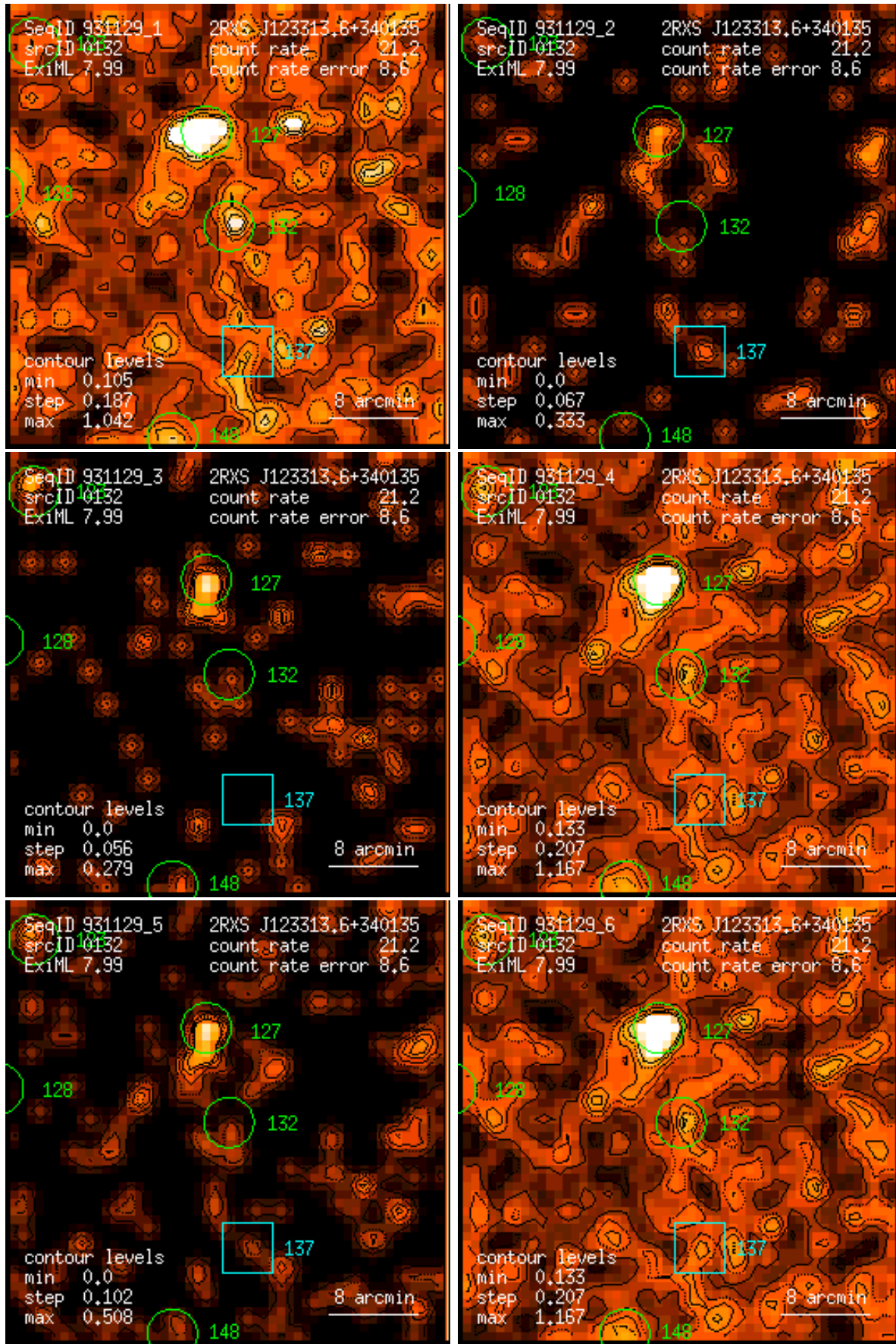
Figure 132: RASS 931129: detection 0132: band rate images, Gaussian filter: (1) PSPC channels 11 – 41, (2) 52 – 90, (3) 91 – 201, (4) 11 – 235, (5) 52 – 201, (6) 11 – 201. Broad band rates in counts/ks. Band rate contour levels in counts/ks/arcmin 2 .
