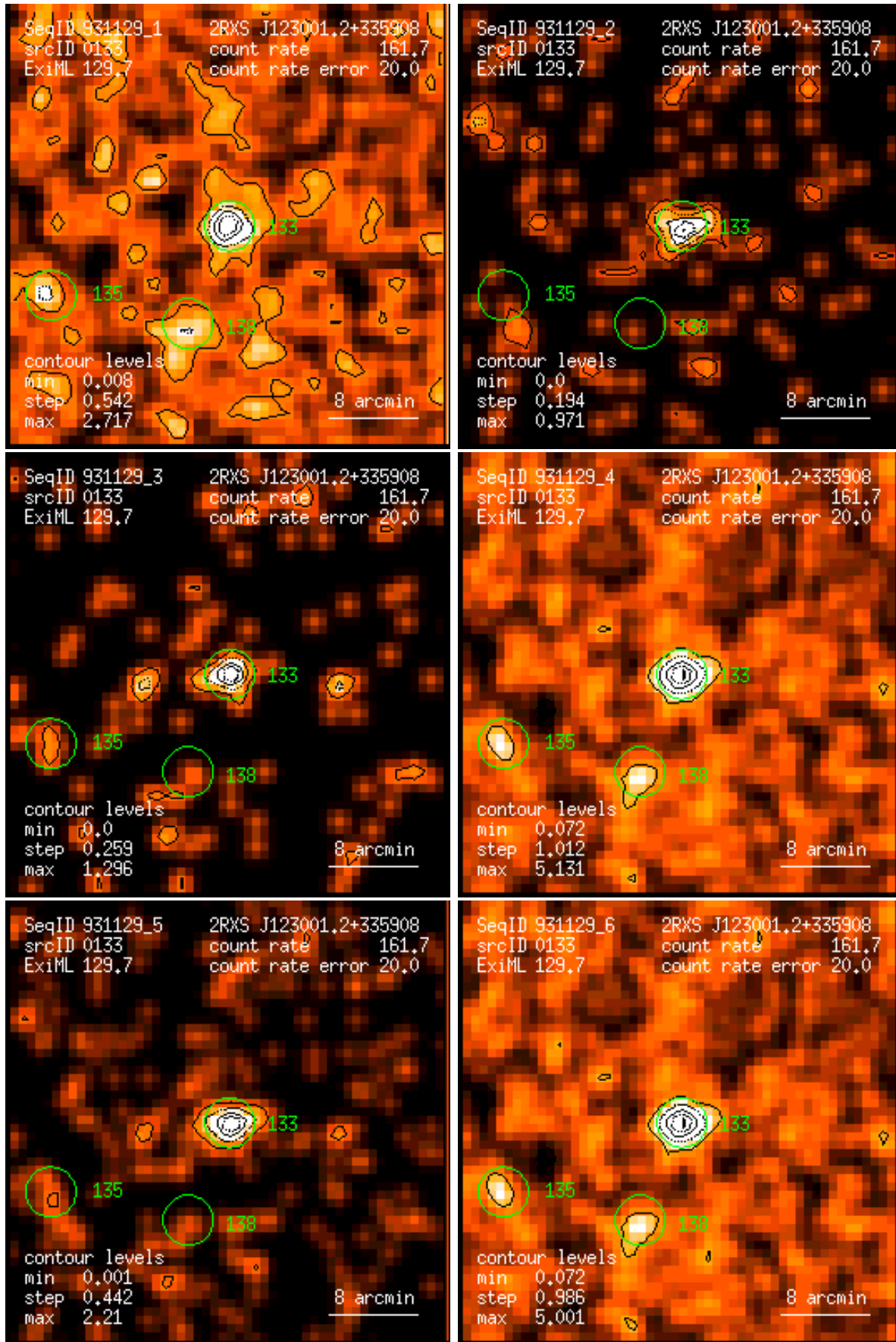
Figure 133: RASS 931129: detection 0133: band rate images, Gaussian filter: (1) PSPC channels 11 – 41, (2) 52 – 90, (3) 91 – 201, (4) 11 – 235, (5) 52 – 201, (6) 11 – 201. Broad band rates in counts/ks. Band rate contour levels in counts/ks/arcmin 2 .
