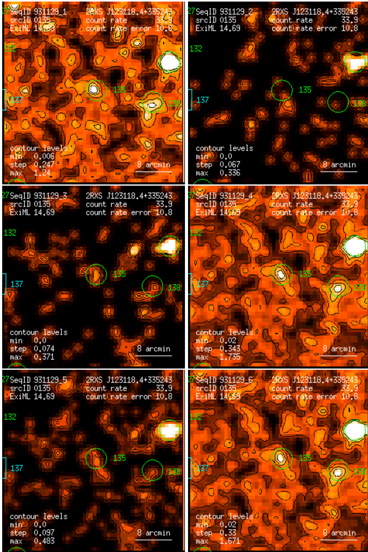
Figure 135: RASS 931129: detection 0135: band rate images, Gaussian filter: (1) PSPC channels 11 – 41, (2) 52 – 90, (3) 91 – 201, (4) 11 – 235, (5) 52 – 201, (6) 11 – 201. Broad band rates in counts/ks. Band rate contour levels in counts/ks/arcmin 2 .
