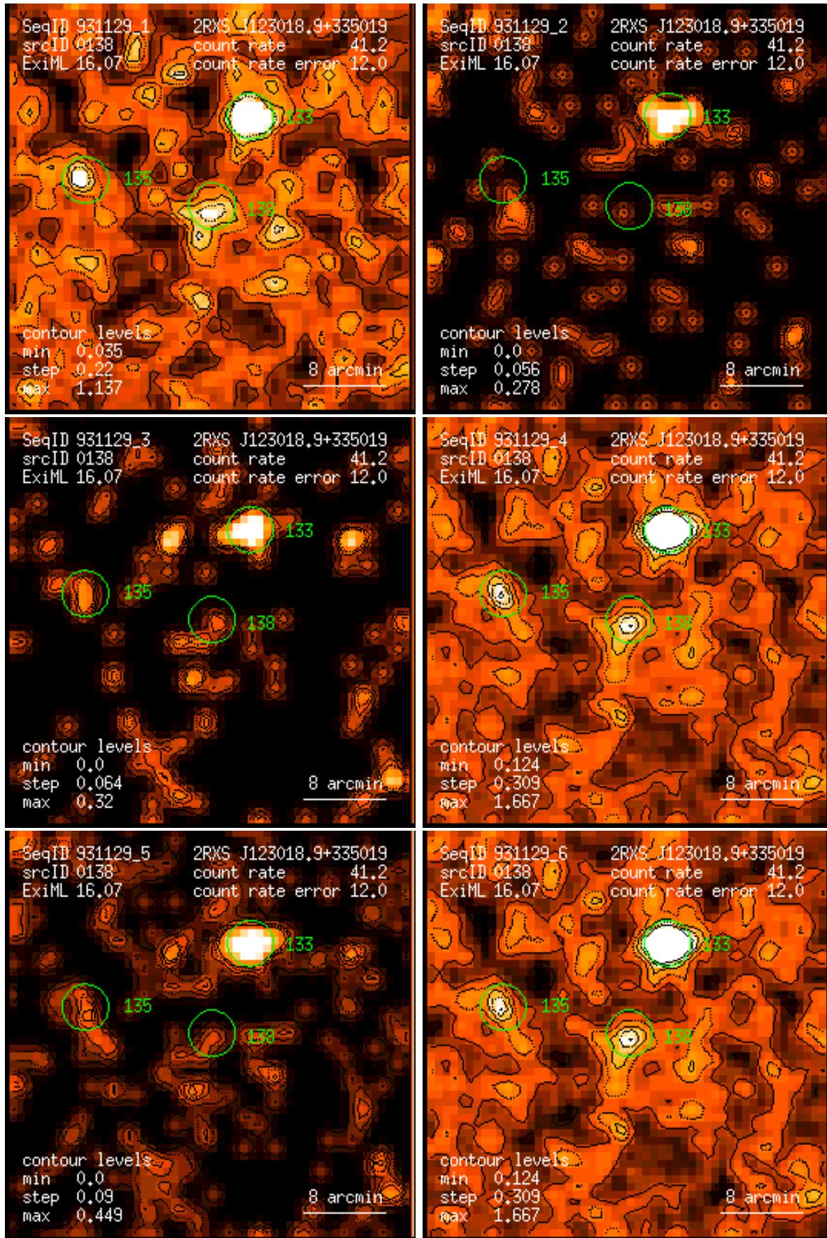
Figure 138: RASS 931129: detection 0138: band rate images, Gaussian filter: (1) PSPC channels 11 – 41, (2) 52 – 90, (3) 91 – 201, (4) 11 – 235, (5) 52 – 201, (6) 11 – 201. Broad band rates in counts/ks. Band rate contour levels in counts/ks/arcmin 2 .
