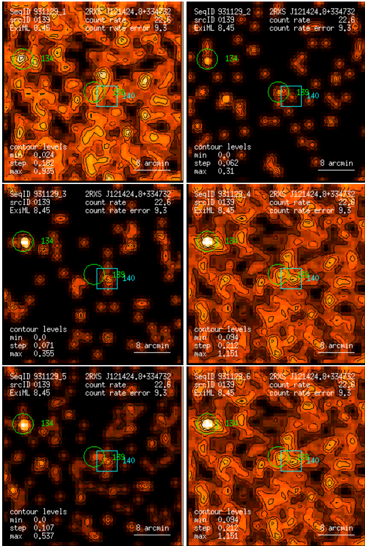
Figure 139: RASS 931129: detection 0139: band rate images, Gaussian filter: (1) PSPC channels 11 – 41, (2) 52 – 90, (3) 91 – 201, (4) 11 – 235, (5) 52 – 201, (6) 11 – 201. Broad band rates in counts/ks. Band rate contour levels in counts/ks/arcmin 2 .
