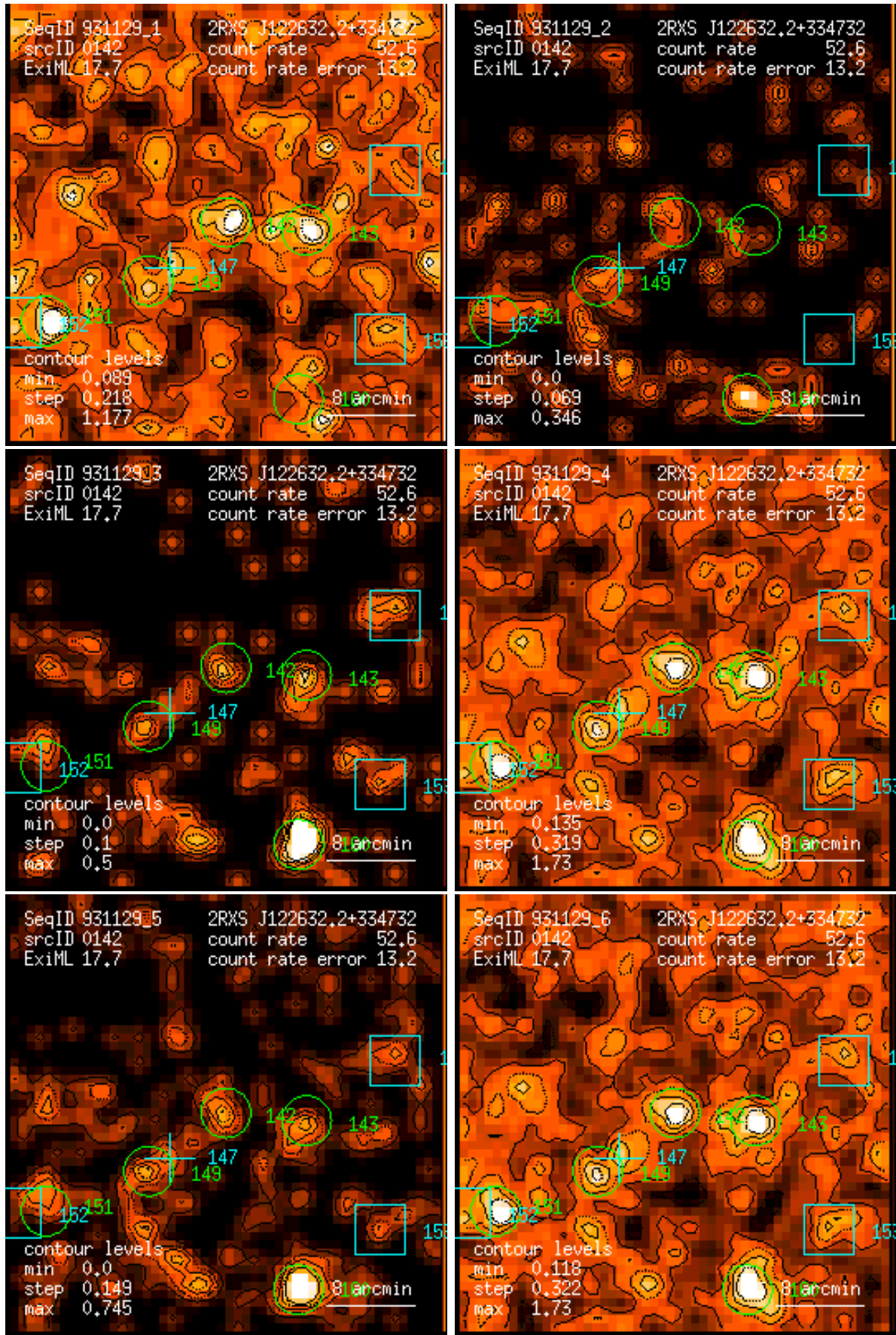
Figure 142: RASS 931129: detection 0142: band rate images, Gaussian filter: (1) PSPC channels 11 – 41, (2) 52 – 90, (3) 91 – 201, (4) 11 – 235, (5) 52 – 201, (6) 11 – 201. Broad band rates in counts/ks. Band rate contour levels in counts/ks/arcmin 2 .
