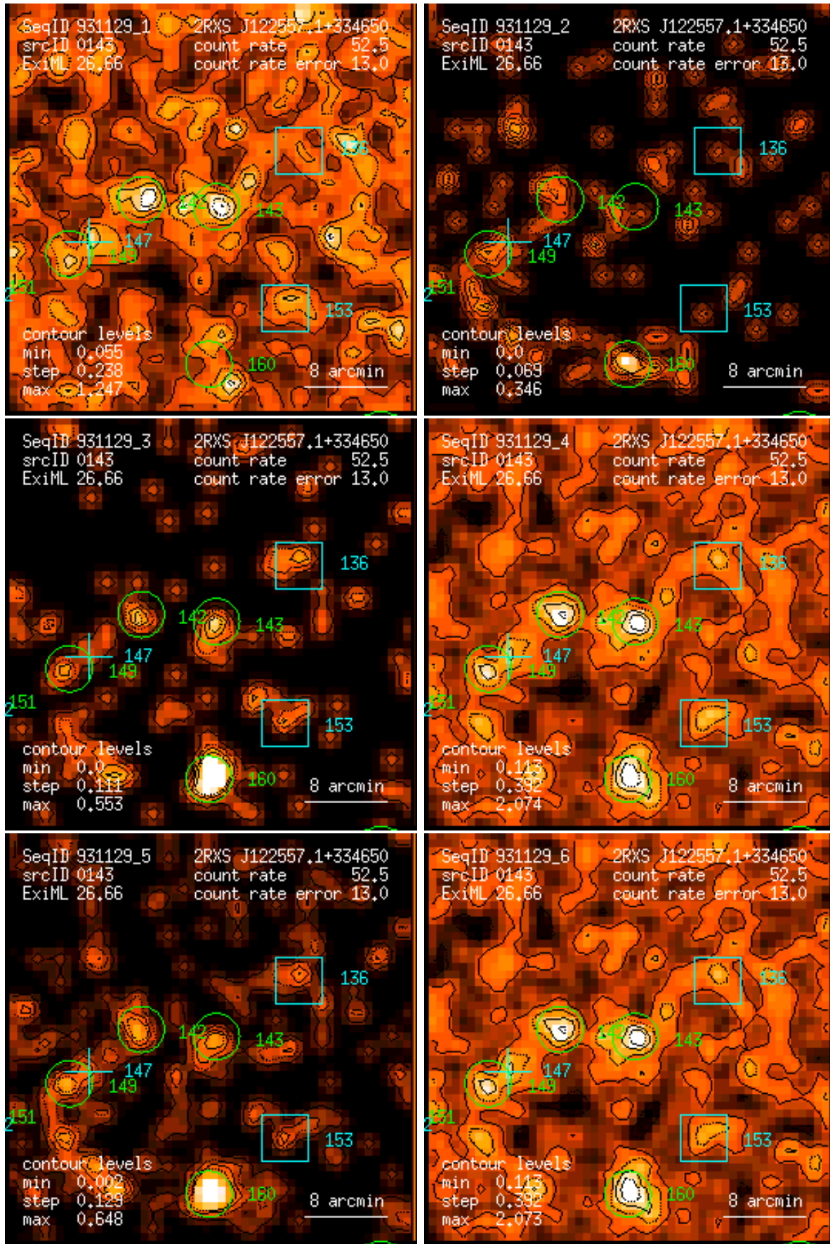
Figure 143: RASS 931129: detection 0143: band rate images, Gaussian filter: (1) PSPC channels 11 – 41, (2) 52 – 90, (3) 91 – 201, (4) 11 – 235, (5) 52 – 201, (6) 11 – 201. Broad band rates in counts/ks. Band rate contour levels in counts/ks/arcmin 2 .
