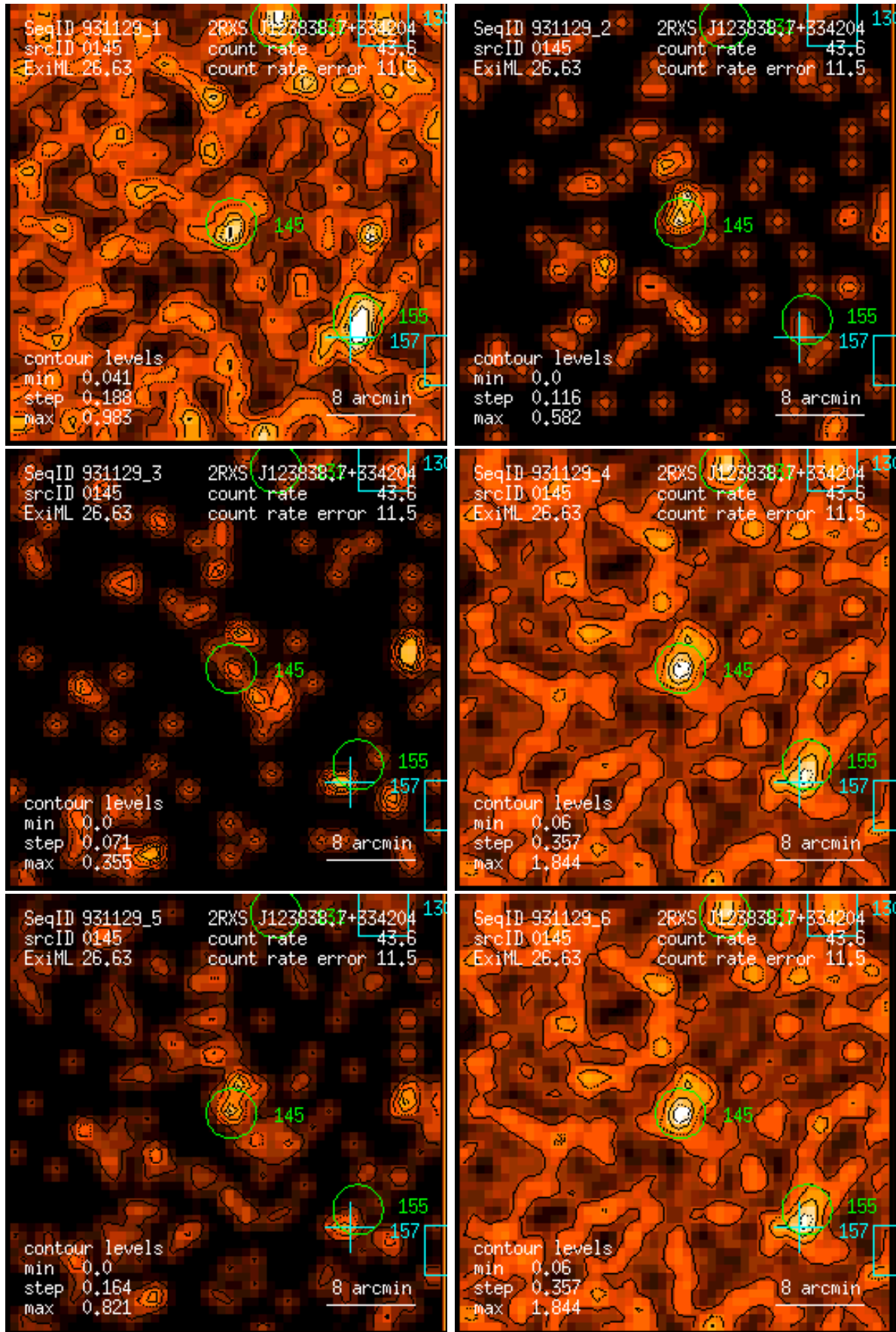
Figure 145: RASS 931129: detection 0145: band rate images, Gaussian filter: (1) PSPC channels 11 – 41, (2) 52 – 90, (3) 91 – 201, (4) 11 – 235, (5) 52 – 201, (6) 11 – 201. Broad band rates in counts/ks. Band rate contour levels in counts/ks/arcmin 2 .
