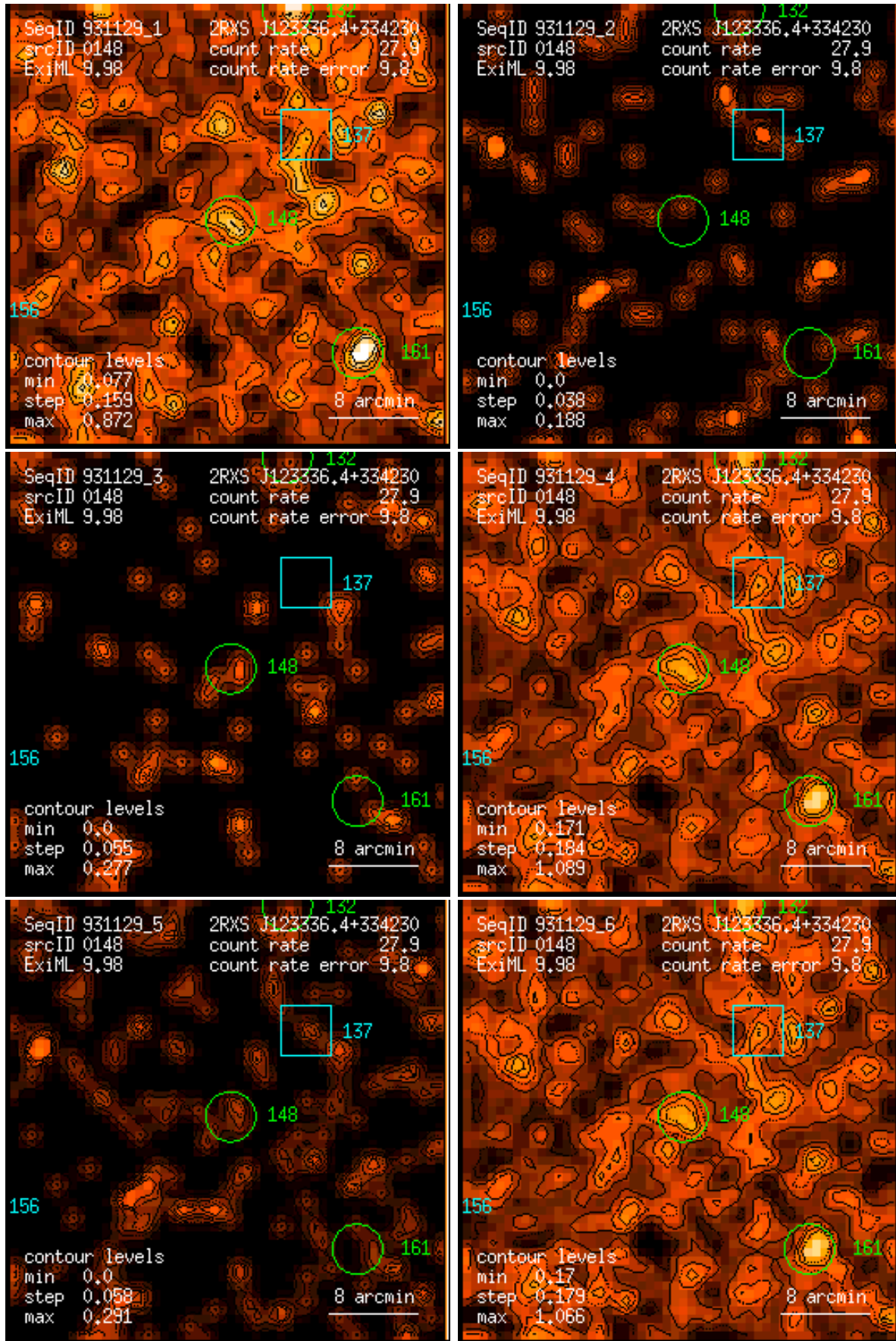
Figure 148: RASS 931129: detection 0148: band rate images, Gaussian filter: (1) PSPC channels 11 – 41, (2) 52 – 90, (3) 91 – 201, (4) 11 – 235, (5) 52 – 201, (6) 11 – 201. Broad band rates in counts/ks. Band rate contour levels in counts/ks/arcmin 2 .
