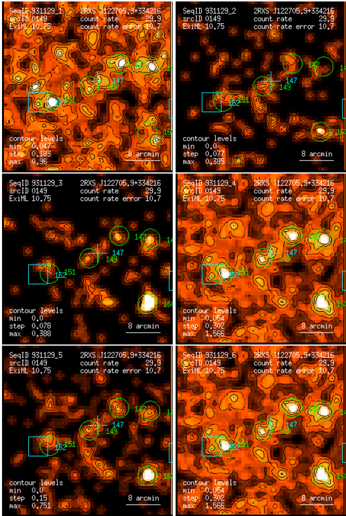
Figure 149: RASS 931129: detection 0149: band rate images, Gaussian filter: (1) PSPC channels 11 – 41, (2) 52 – 90, (3) 91 – 201, (4) 11 – 235, (5) 52 – 201, (6) 11 – 201. Broad band rates in counts/ks. Band rate contour levels in counts/ks/arcmin 2 .
