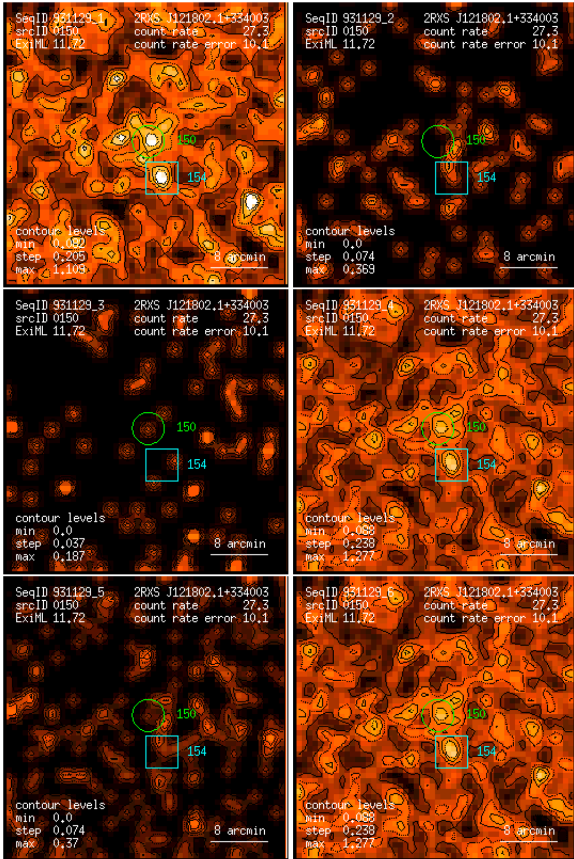
Figure 150: RASS 931129: detection 0150: band rate images, Gaussian filter: (1) PSPC channels 11 – 41, (2) 52 – 90, (3) 91 – 201, (4) 11 – 235, (5) 52 – 201, (6) 11 – 201. Broad band rates in counts/ks. Band rate contour levels in counts/ks/arcmin 2 .
