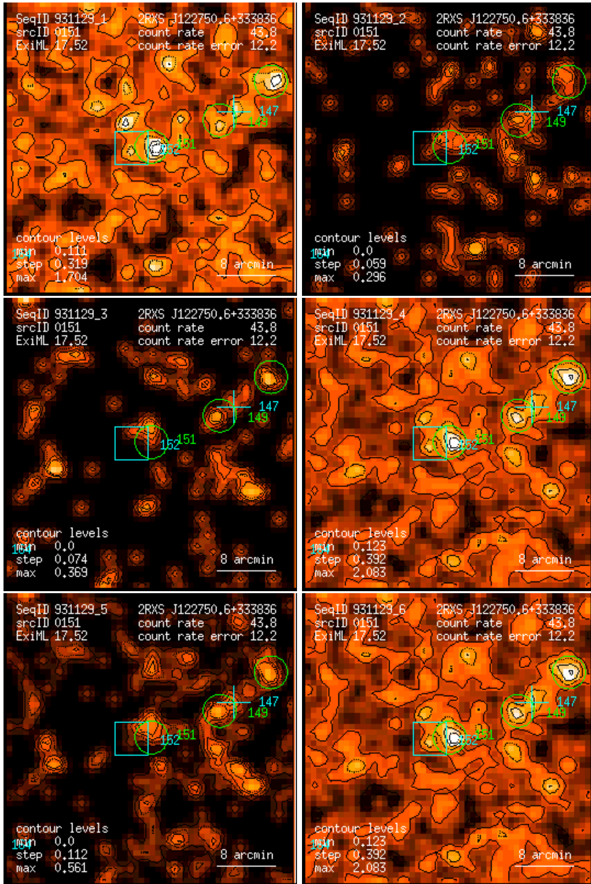
Figure 151: RASS 931129: detection 0151: band rate images, Gaussian filter: (1) PSPC channels 11 – 41, (2) 52 – 90, (3) 91 – 201, (4) 11 – 235, (5) 52 – 201, (6) 11 – 201. Broad band rates in counts/ks. Band rate contour levels in counts/ks/arcmin 2 .
