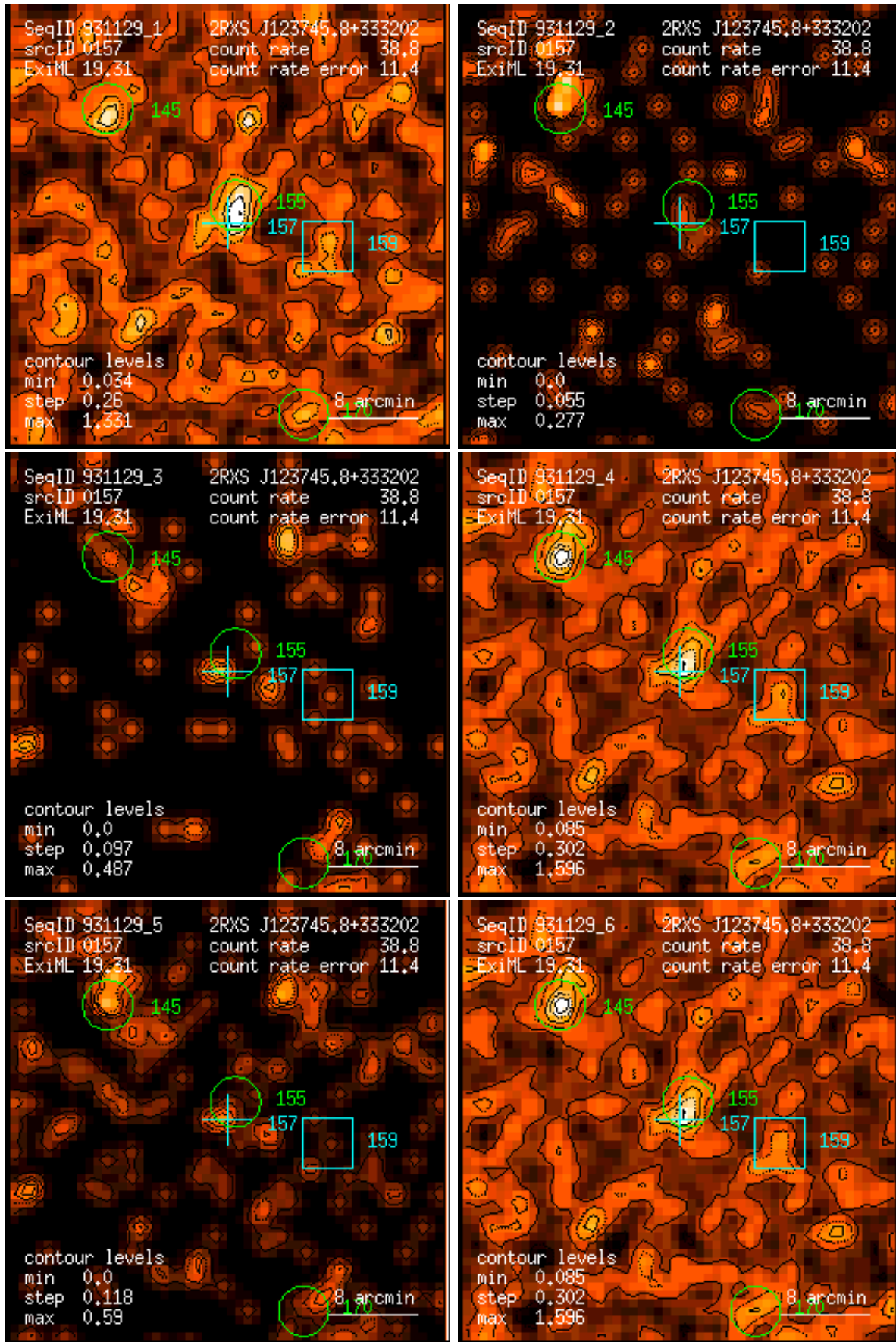
Figure 157: RASS 931129: detection 0157: band rate images, Gaussian filter: (1) PSPC channels 11 – 41, (2) 52 – 90, (3) 91 – 201, (4) 11 – 235, (5) 52 – 201, (6) 11 – 201. Broad band rates in counts/ks. Band rate contour levels in counts/ks/arcmin 2 .
