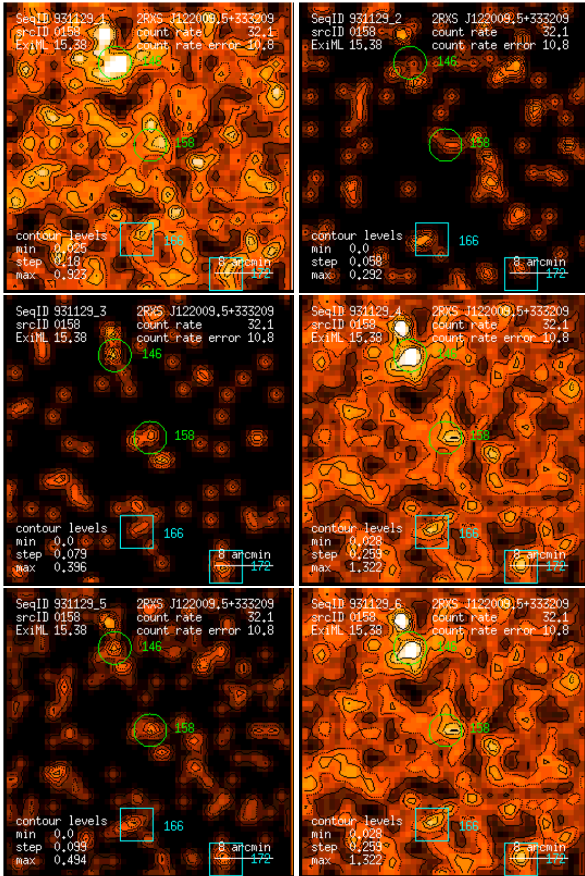
Figure 158: RASS 931129: detection 0158: band rate images, Gaussian filter: (1) PSPC channels 11 – 41, (2) 52 – 90, (3) 91 – 201, (4) 11 – 235, (5) 52 – 201, (6) 11 – 201. Broad band rates in counts/ks. Band rate contour levels in counts/ks/arcmin 2 .
