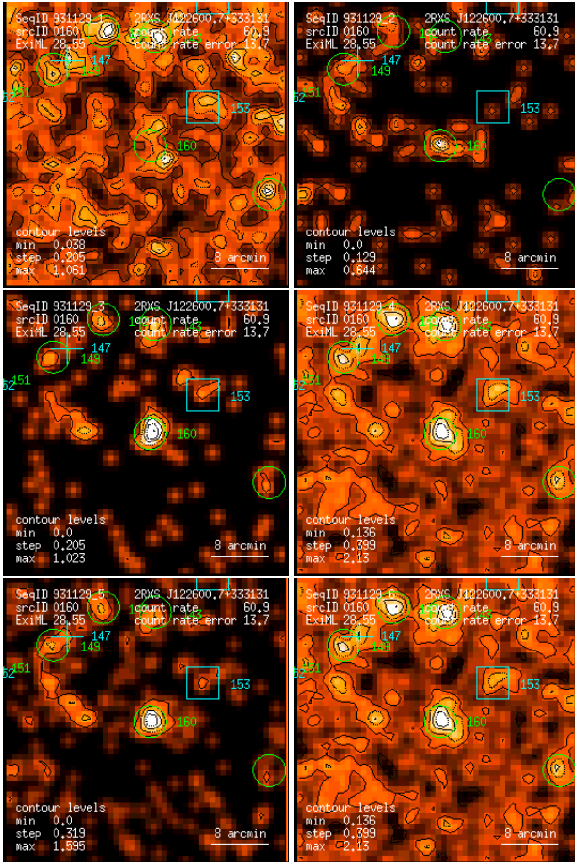
Figure 160: RASS 931129: detection 0160: band rate images, Gaussian filter: (1) PSPC channels 11 – 41, (2) 52 – 90, (3) 91 – 201, (4) 11 – 235, (5) 52 – 201, (6) 11 – 201. Broad band rates in counts/ks. Band rate contour levels in counts/ks/arcmin 2 .
