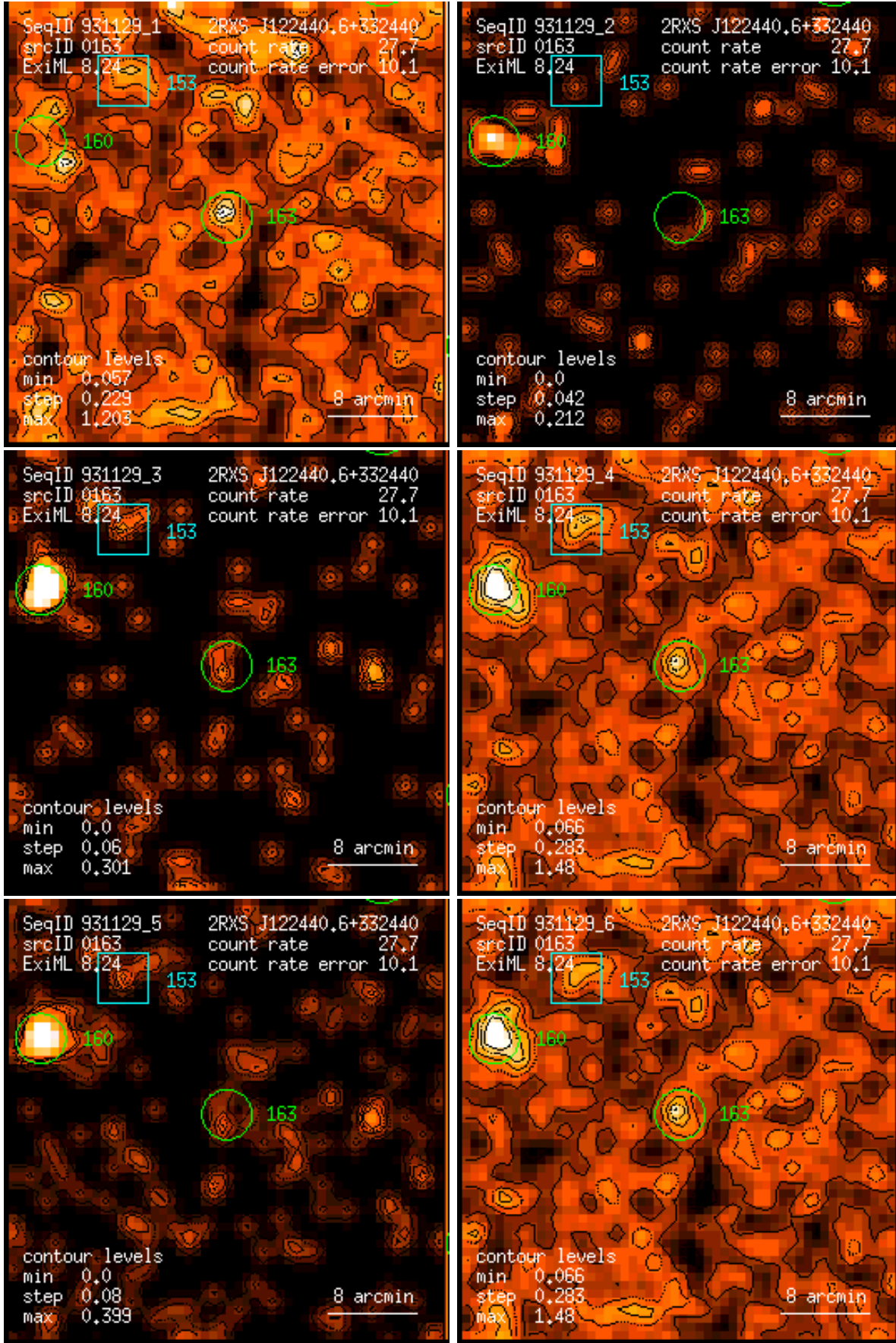
Figure 163: RASS 931129: detection 0163: band rate images, Gaussian filter: (1) PSPC channels 11 – 41, (2) 52 – 90, (3) 91 – 201, (4) 11 – 235, (5) 52 – 201, (6) 11 – 201. Broad band rates in counts/ks. Band rate contour levels in counts/ks/arcmin 2 .
