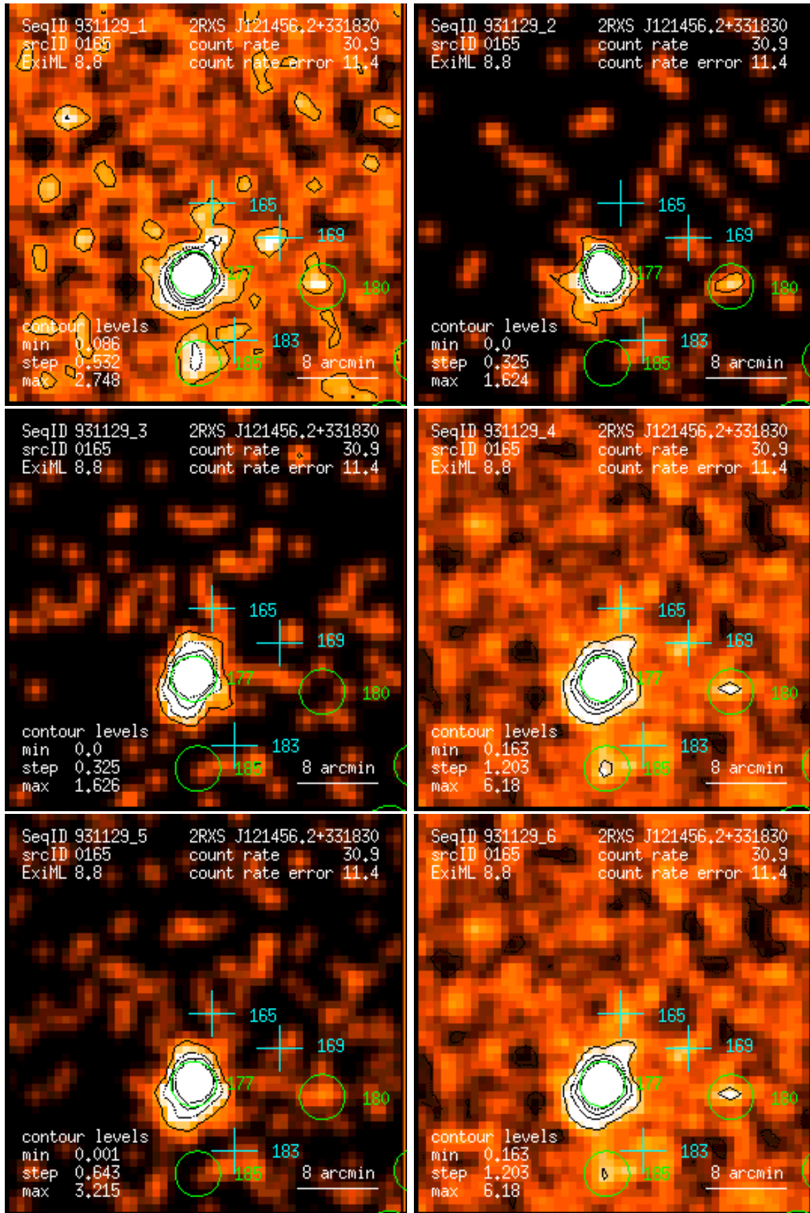
Figure 165: RASS 931129: detection 0165: band rate images, Gaussian filter: (1) PSPC channels 11 – 41, (2) 52 – 90, (3) 91 – 201, (4) 11 – 235, (5) 52 – 201, (6) 11 – 201. Broad band rates in counts/ks. Band rate contour levels in counts/ks/arcmin 2 .
