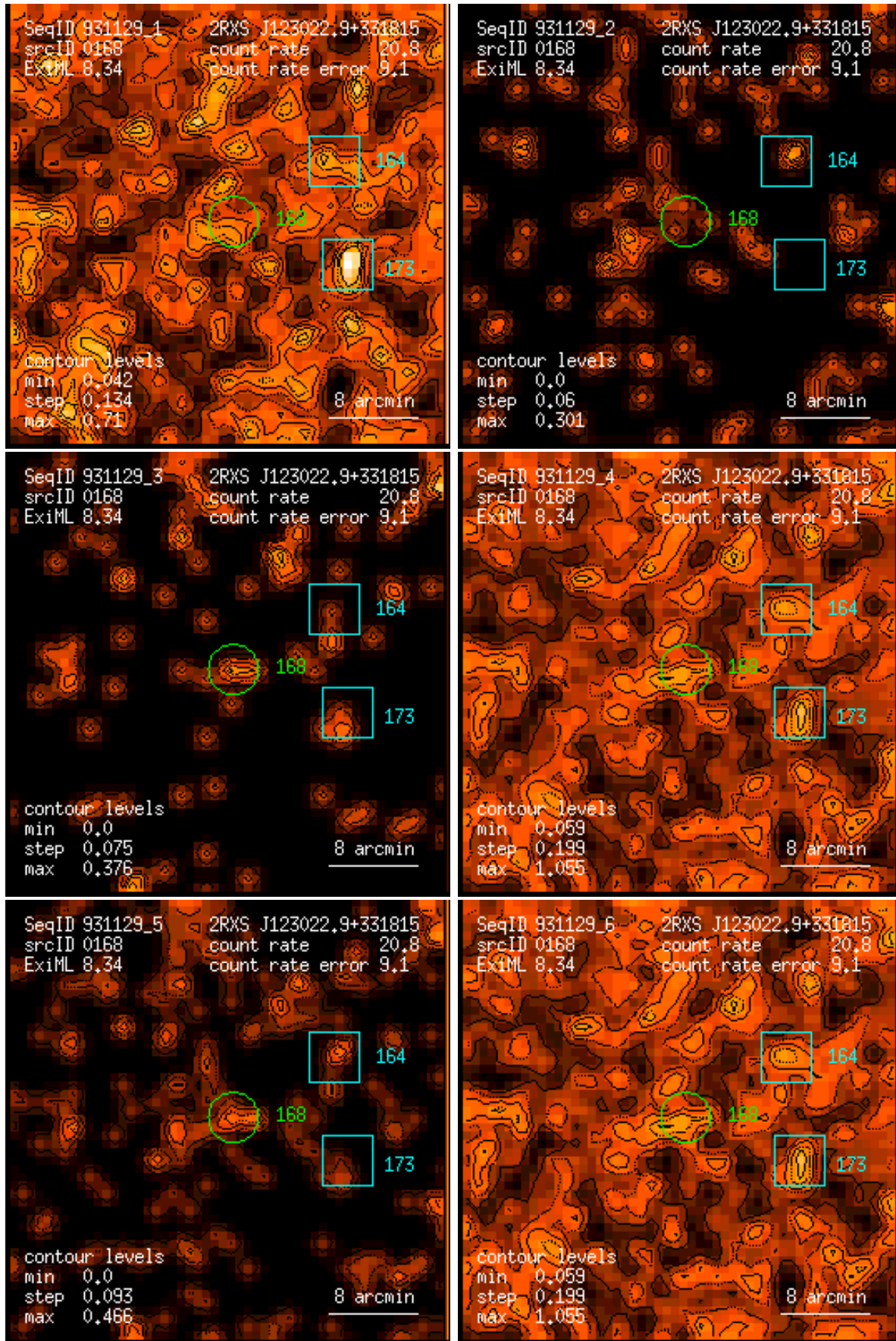
Figure 168: RASS 931129: detection 0168: band rate images, Gaussian filter: (1) PSPC channels 11 – 41, (2) 52 – 90, (3) 91 – 201, (4) 11 – 235, (5) 52 – 201, (6) 11 – 201. Broad band rates in counts/ks. Band rate contour levels in counts/ks/arcmin 2 .
