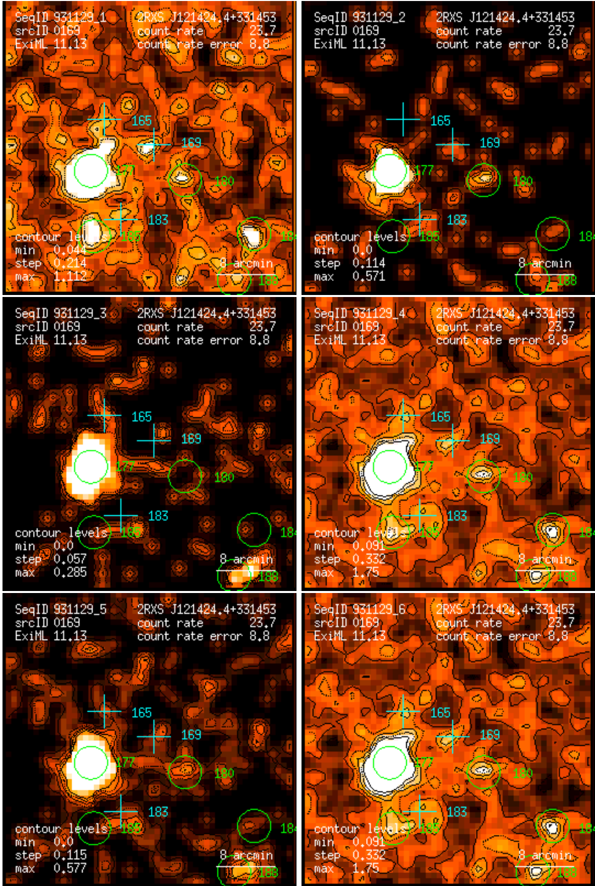
Figure 169: RASS 931129: detection 0169: band rate images, Gaussian filter: (1) PSPC channels 11 – 41, (2) 52 – 90, (3) 91 – 201, (4) 11 – 235, (5) 52 – 201, (6) 11 – 201. Broad band rates in counts/ks. Band rate contour levels in counts/ks/arcmin 2 .
