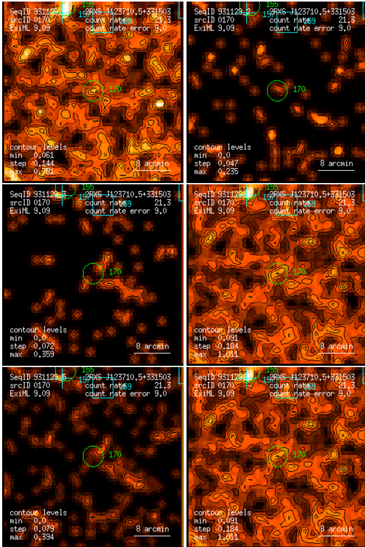
Figure 170: RASS 931129: detection 0170: band rate images, Gaussian filter: (1) PSPC channels 11 – 41, (2) 52 – 90, (3) 91 – 201, (4) 11 – 235, (5) 52 – 201, (6) 11 – 201. Broad band rates in counts/ks. Band rate contour levels in counts/ks/arcmin 2 .
