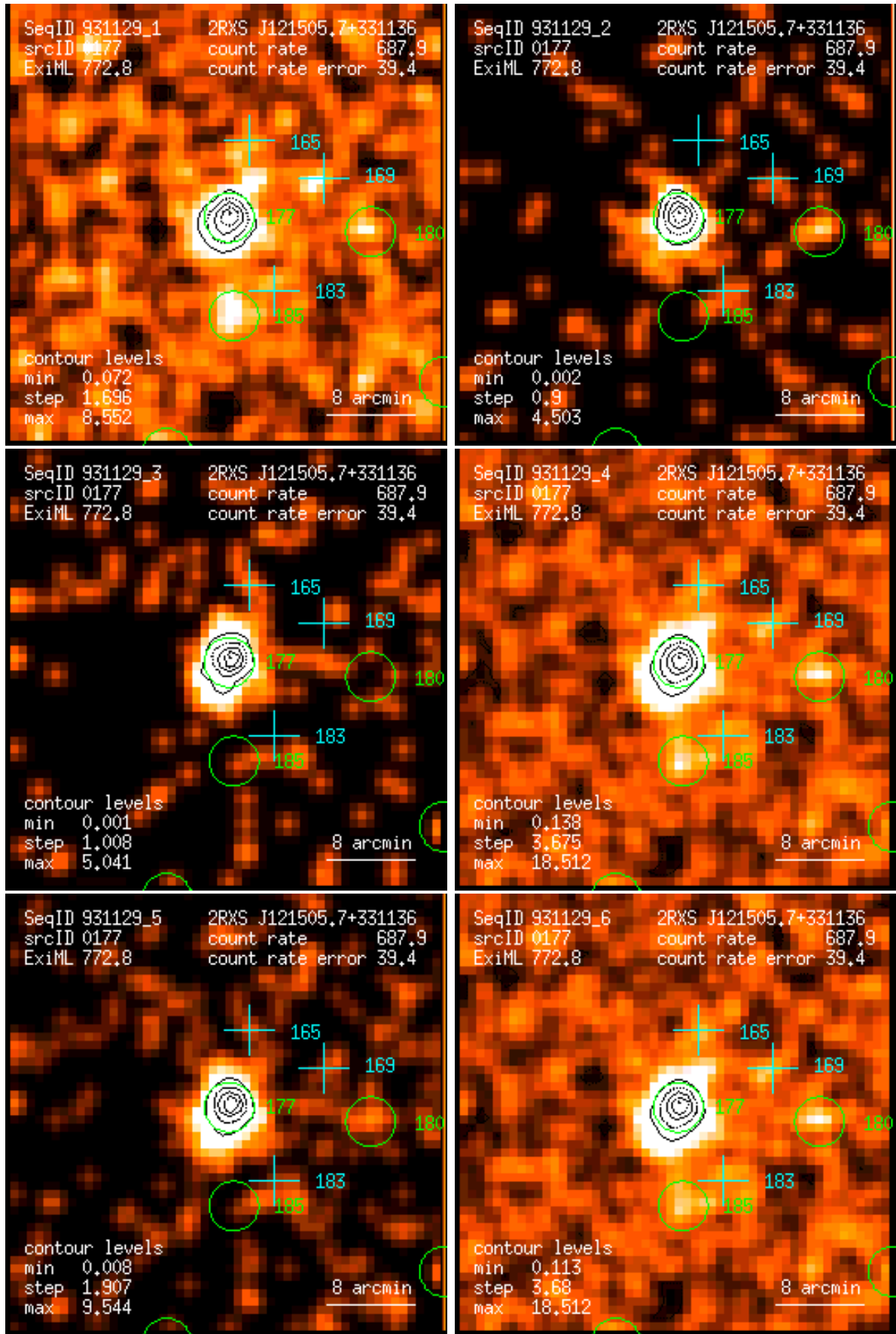
Figure 177: RASS 931129: detection 0177: band rate images, Gaussian filter: (1) PSPC channels 11 – 41, (2) 52 – 90, (3) 91 – 201, (4) 11 – 235, (5) 52 – 201, (6) 11 – 201. Broad band rates in counts/ks. Band rate contour levels in counts/ks/arcmin 2 .
