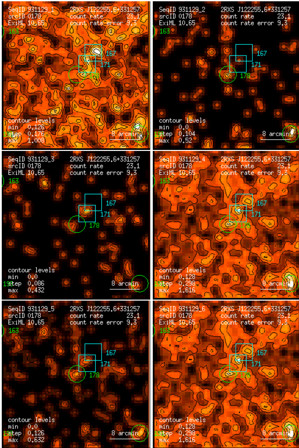
Figure 178: RASS 931129: detection 0178: band rate images, Gaussian filter: (1) PSPC channels 11 – 41, (2) 52 – 90, (3) 91 – 201, (4) 11 – 235, (5) 52 – 201, (6) 11 – 201. Broad band rates in counts/ks. Band rate contour levels in counts/ks/arcmin 2 .
