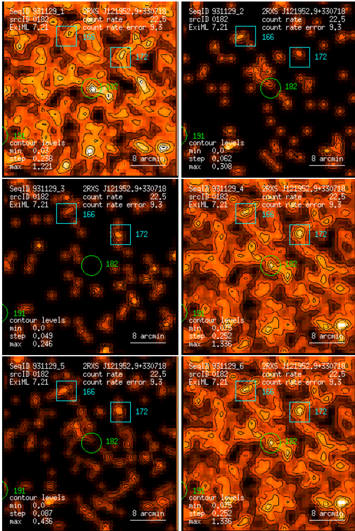
Figure 182: RASS 931129: detection 0182: band rate images, Gaussian filter: (1) PSPC channels 11 – 41, (2) 52 – 90, (3) 91 – 201, (4) 11 – 235, (5) 52 – 201, (6) 11 – 201. Broad band rates in counts/ks. Band rate contour levels in counts/ks/arcmin 2 .
