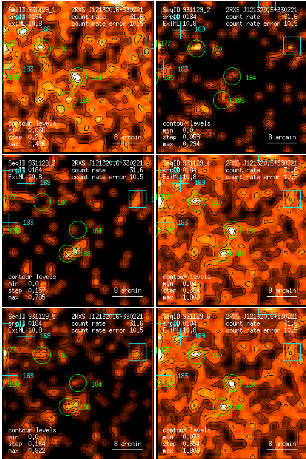
Figure 184: RASS 931129: detection 0184: band rate images, Gaussian filter: (1) PSPC channels 11 – 41, (2) 52 – 90, (3) 91 – 201, (4) 11 – 235, (5) 52 – 201, (6) 11 – 201. Broad band rates in counts/ks. Band rate contour levels in counts/ks/arcmin 2 .
