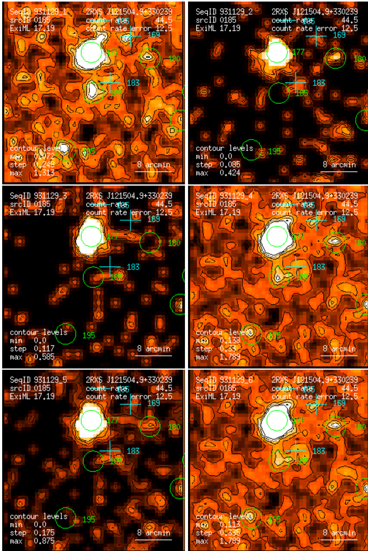
Figure 185: RASS 931129: detection 0185: band rate images, Gaussian filter: (1) PSPC channels 11 – 41, (2) 52 – 90, (3) 91 – 201, (4) 11 – 235, (5) 52 – 201, (6) 11 – 201. Broad band rates in counts/ks. Band rate contour levels in counts/ks/arcmin 2 .
