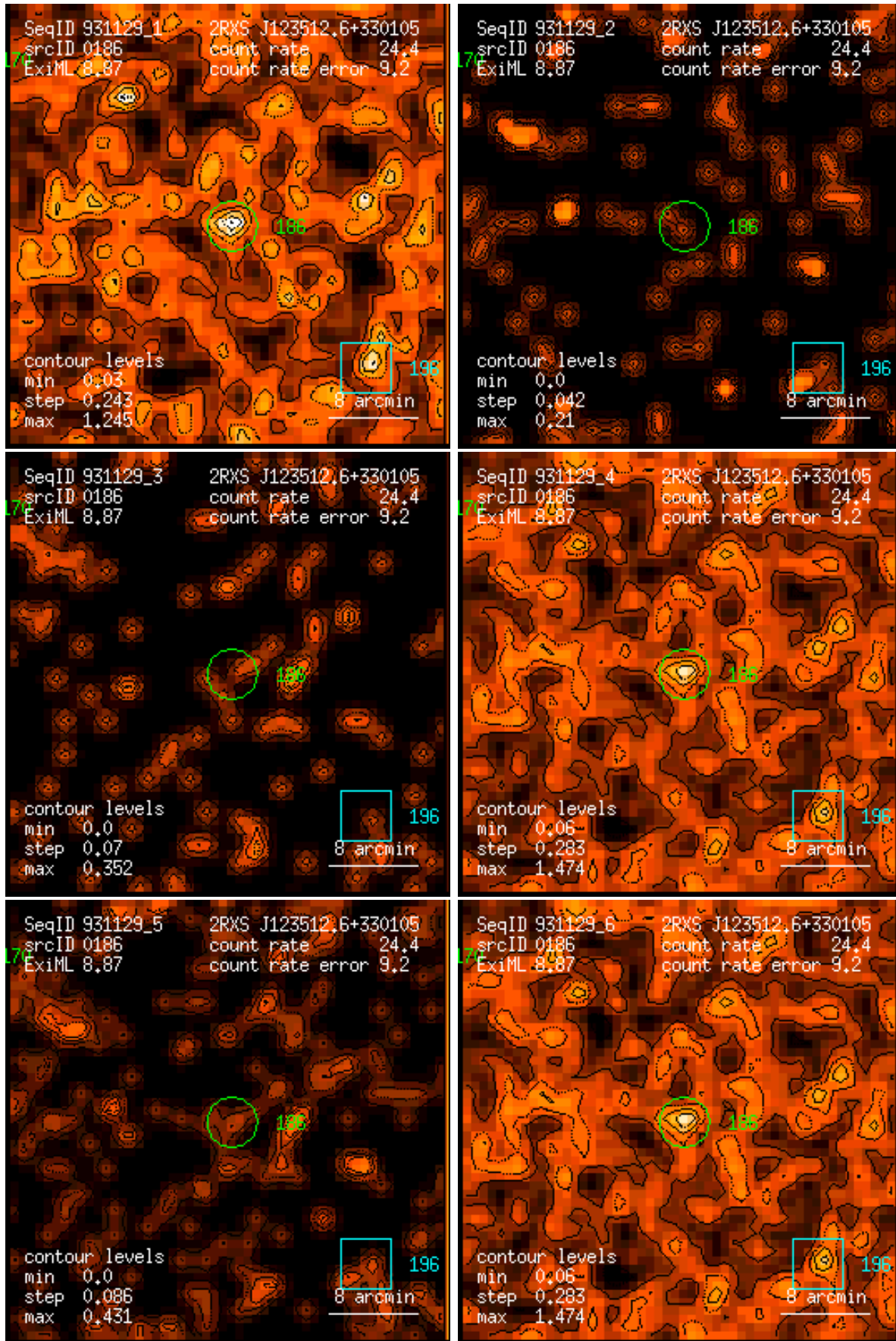
Figure 186: RASS 931129: detection 0186: band rate images, Gaussian filter: (1) PSPC channels 11 – 41, (2) 52 – 90, (3) 91 – 201, (4) 11 – 235, (5) 52 – 201, (6) 11 – 201. Broad band rates in counts/ks. Band rate contour levels in counts/ks/arcmin 2 .
