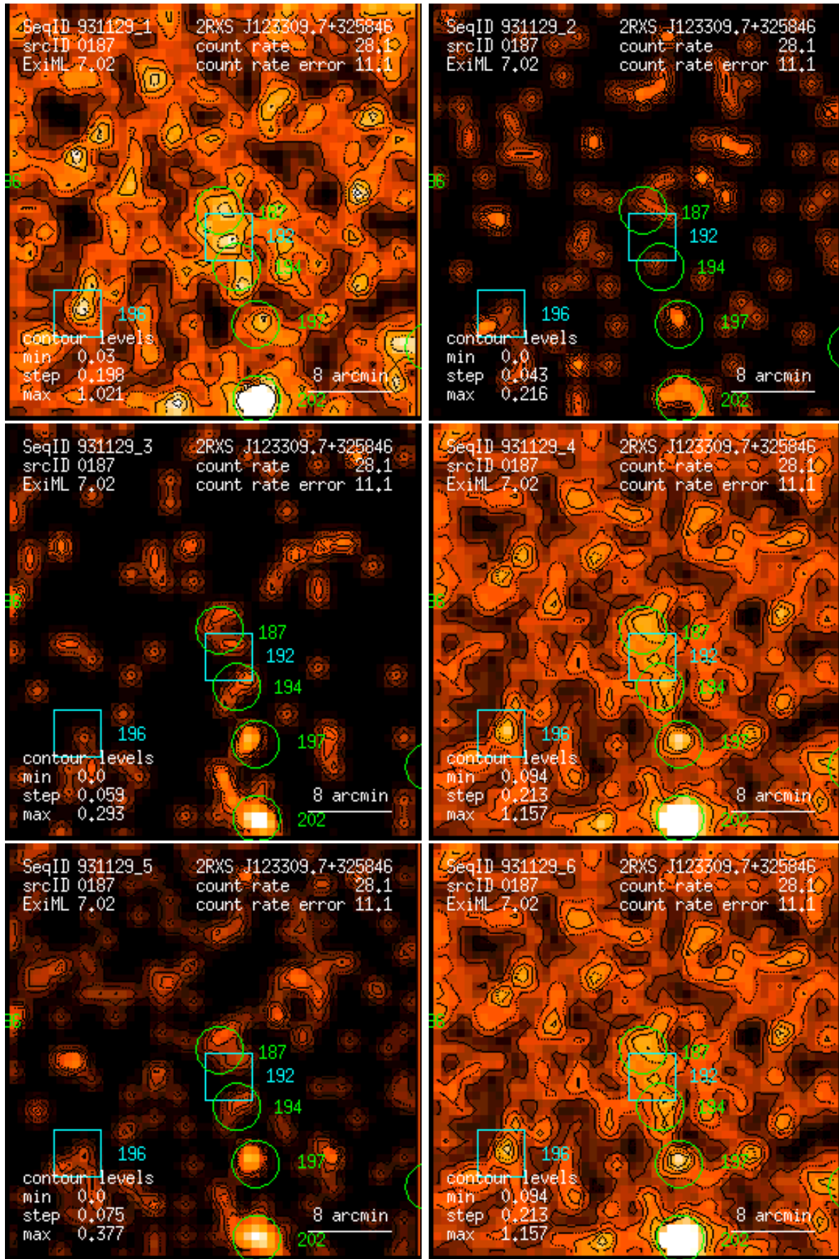
Figure 187: RASS 931129: detection 0187: band rate images, Gaussian filter: (1) PSPC channels 11 – 41, (2) 52 – 90, (3) 91 – 201, (4) 11 – 235, (5) 52 – 201, (6) 11 – 201. Broad band rates in counts/ks. Band rate contour levels in counts/ks/arcmin 2 .
