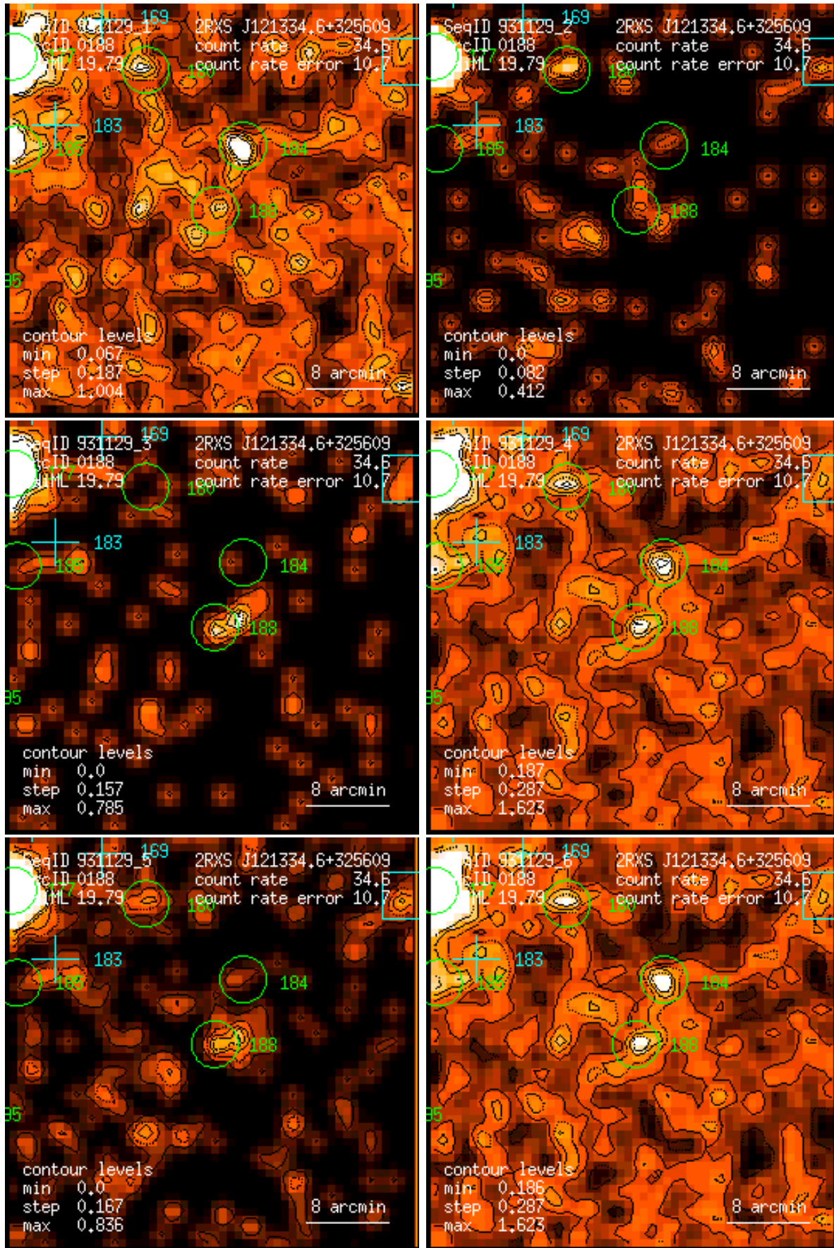
Figure 188: RASS 931129: detection 0188: band rate images, Gaussian filter: (1) PSPC channels 11 – 41, (2) 52 – 90, (3) 91 – 201, (4) 11 – 235, (5) 52 – 201, (6) 11 – 201. Broad band rates in counts/ks. Band rate contour levels in counts/ks/arcmin 2 .
