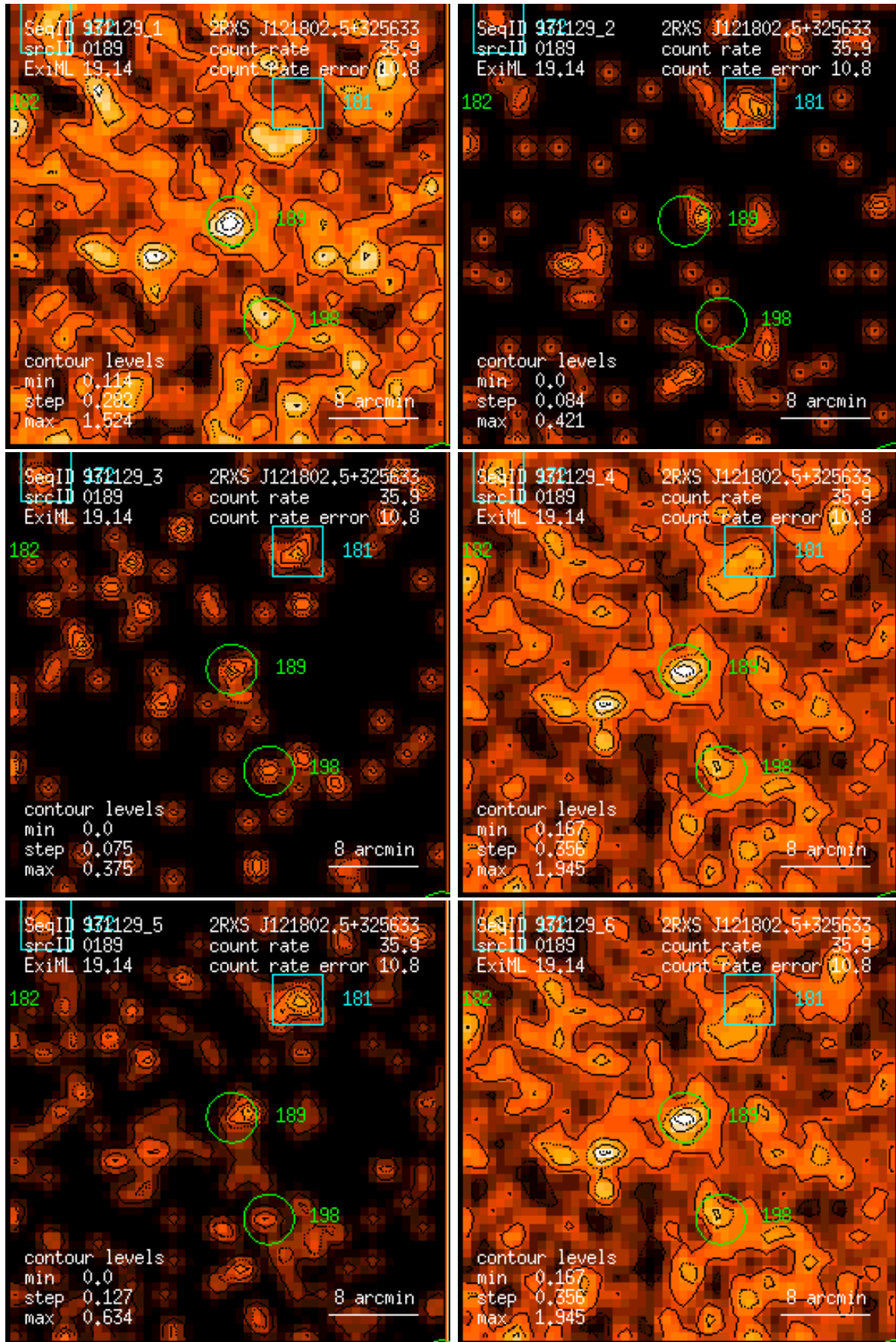
Figure 189: RASS 931129: detection 0189: band rate images, Gaussian filter: (1) PSPC channels 11 – 41, (2) 52 – 90, (3) 91 – 201, (4) 11 – 235, (5) 52 – 201, (6) 11 – 201. Broad band rates in counts/ks. Band rate contour levels in counts/ks/arcmin 2 .
