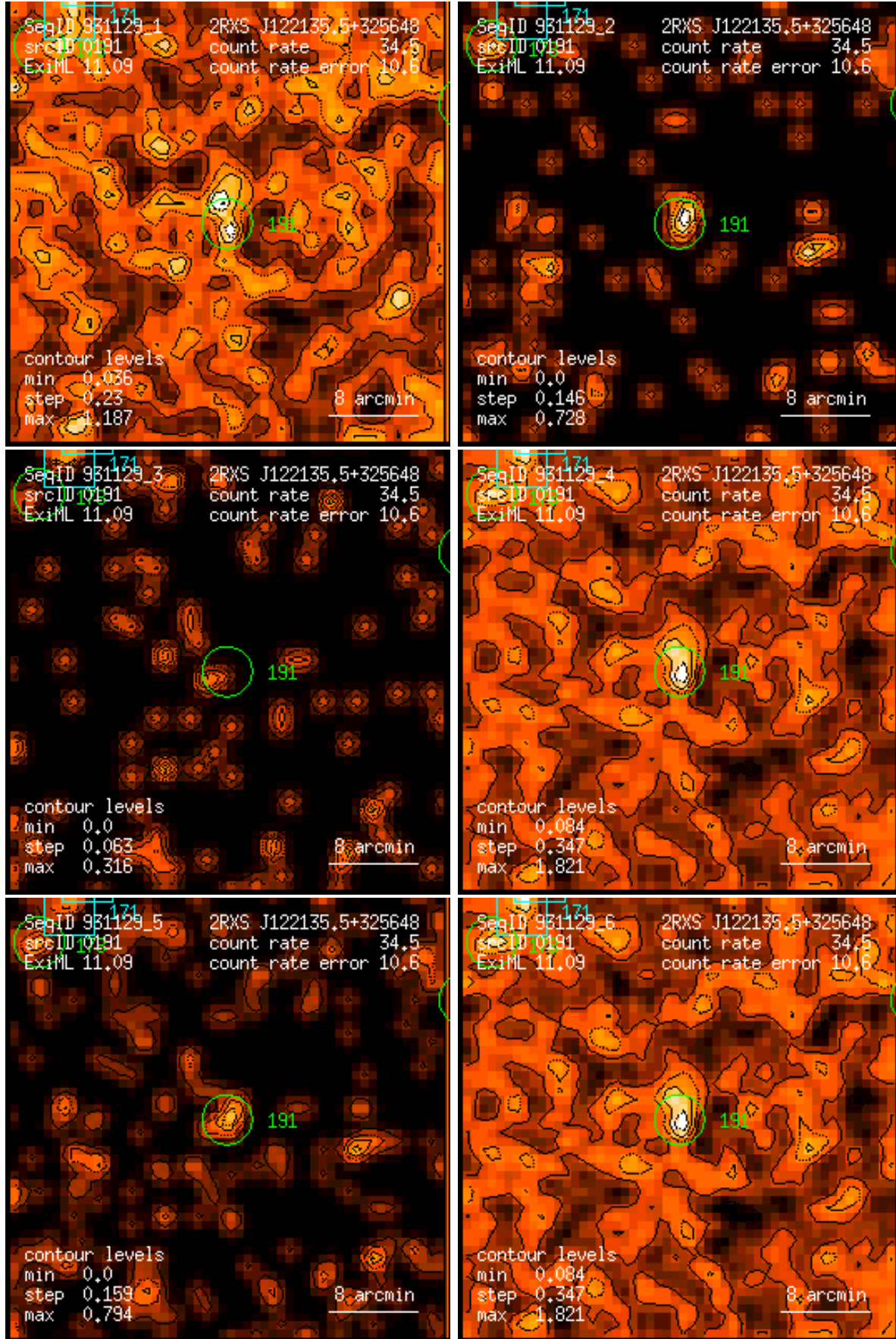
Figure 191: RASS 931129: detection 0191: band rate images, Gaussian filter: (1) PSPC channels 11 – 41, (2) 52 – 90, (3) 91 – 201, (4) 11 – 235, (5) 52 – 201, (6) 11 – 201. Broad band rates in counts/ks. Band rate contour levels in counts/ks/arcmin 2 .
