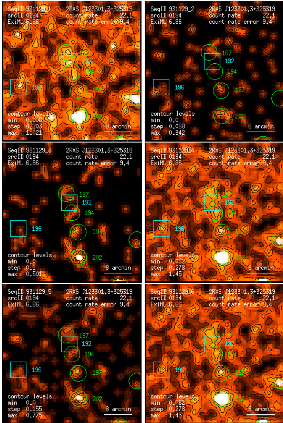
Figure 194: RASS 931129: detection 0194: band rate images, Gaussian filter: (1) PSPPC channels 11 – 41, (2) 52 – 90, (3) 91 – 201, (4) 11 – 235, (5) 52 – 201, (6) 11 – 201. Broad band rates in counts/ks. Band rate contour levels in counts/ks/arcmin 2 .
